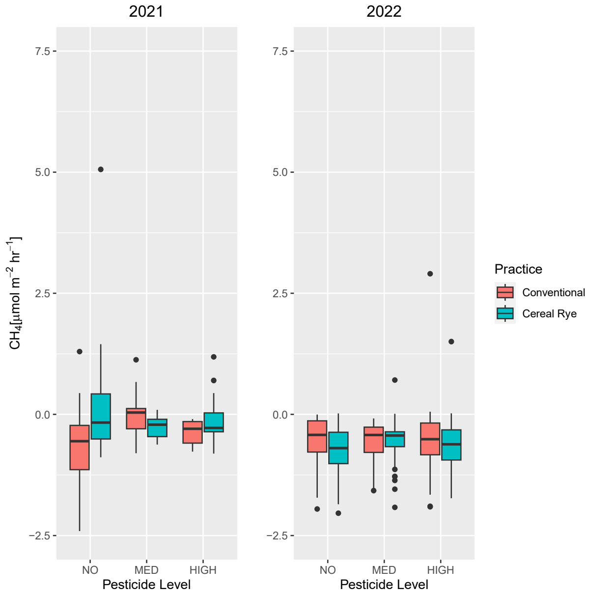
Figure 4. Soil CH 4 fluxes in directly fertilized plots excluding Plot 202 for each type of agricultural practices (conventional in red and cereal rye in green) and pesticide input levels (no, med, and high) in 2021
