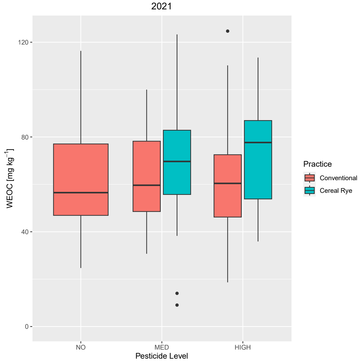
Figure 2. WEOC in non-directly fertilized plots for each type of agricultural practices (conventional in red and cereal rye in green) and pesticide input levels (no, med, and high) in 2021
