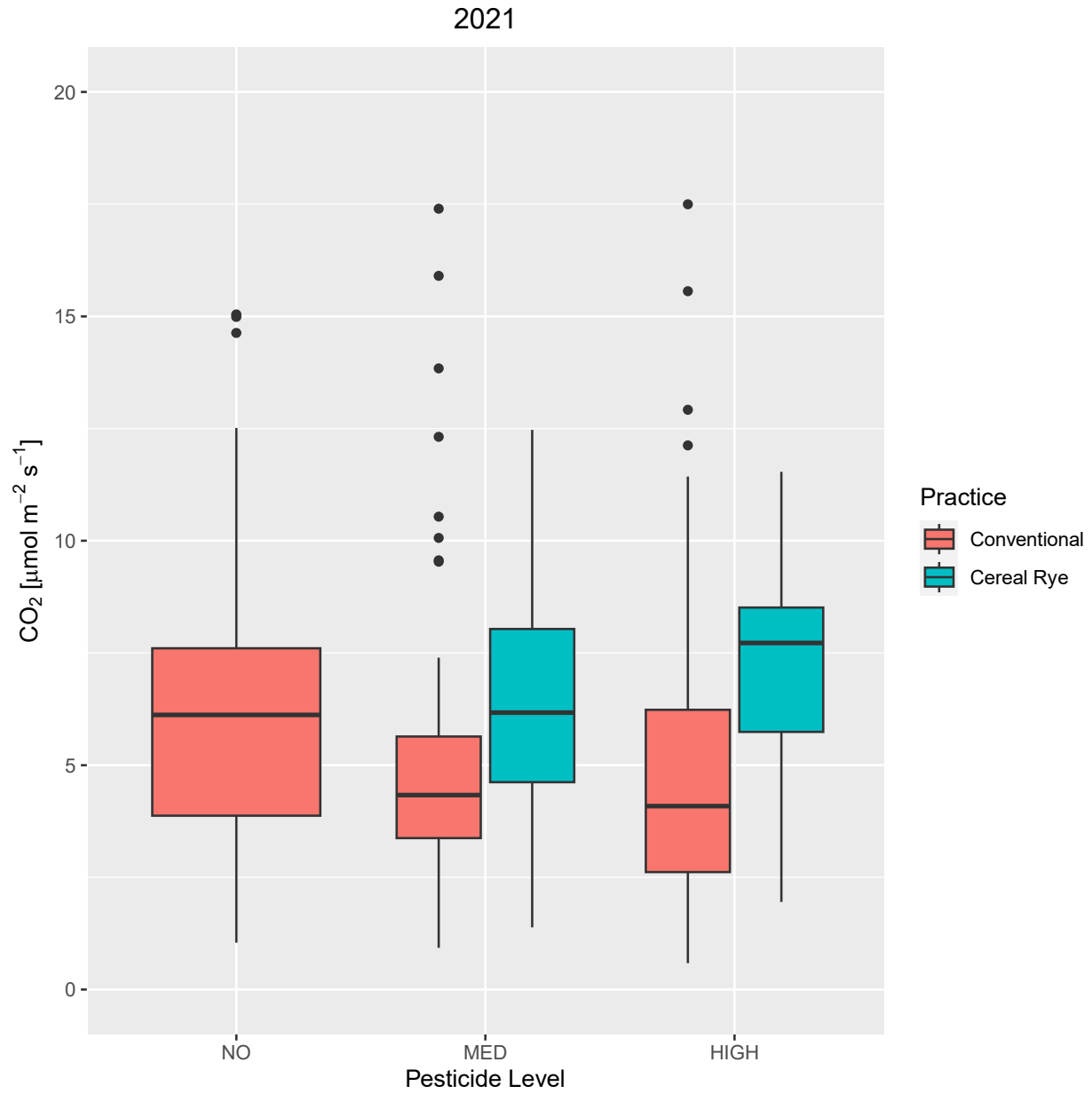
Figure 3. Soil CO 2 fluxes in non-directly fertilized plots for each type of agricultural practices (conventional in red and cereal rye in green) and pesticide input levels (no, med, and high) in 2021
