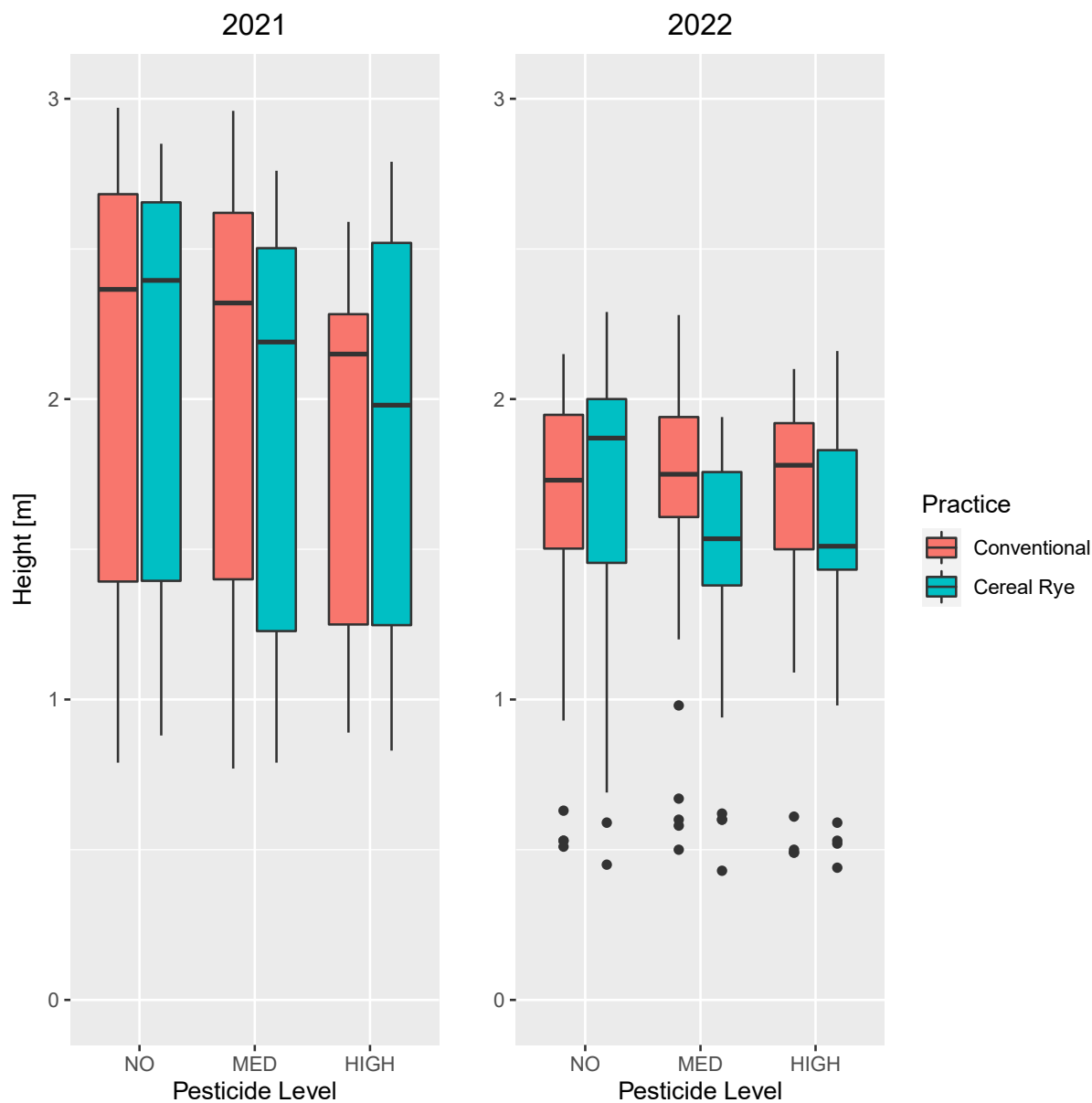
Figure 1. Corn height [m] in 2021 (left) and 2022 (right) for conventional plots (red); and for cereal rye cover crop plots (green).
