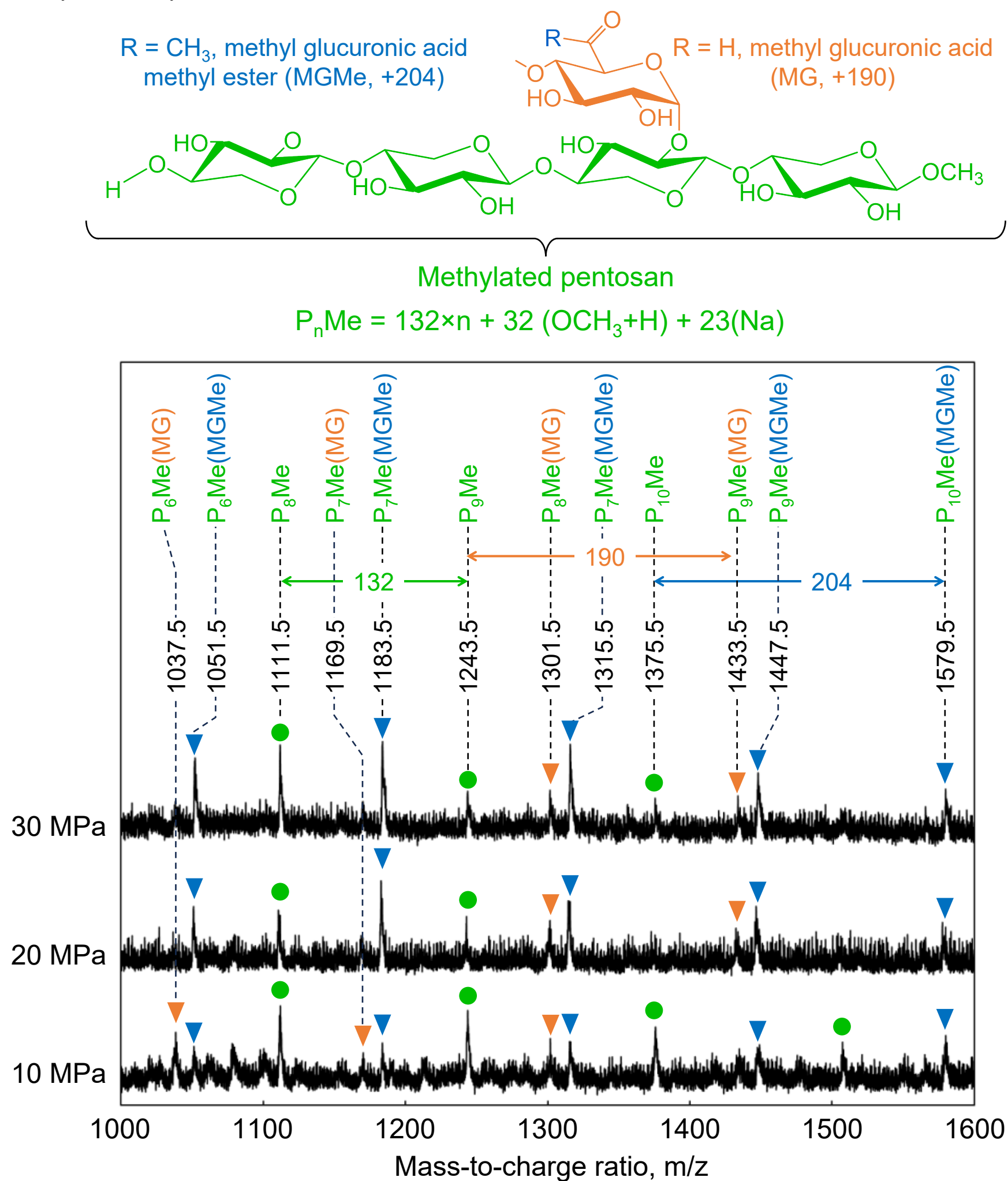
Figure 8. Matrix-assisted laser desorption ionization-time-of-flight mass spectra of oligosaccharides obtained from holocellulose after treatment with methanol/water (90/10, v/v) at various pressures.
