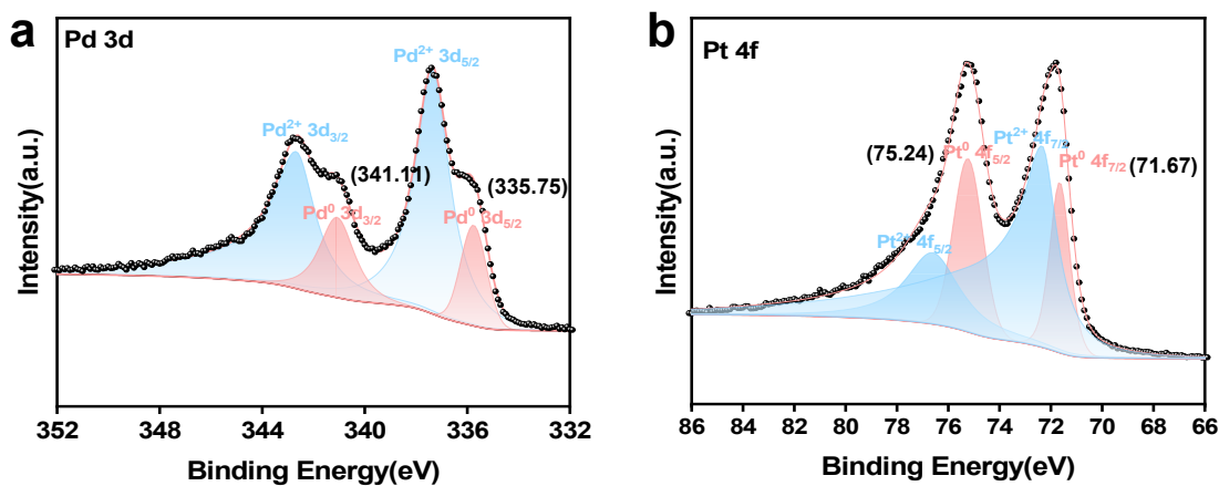
Figure S2. XPS spectra of the commercial catalysts: (a) Pd and (b) Pt.
