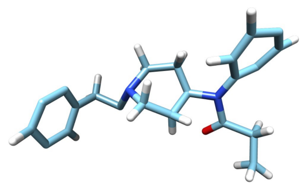
state -1 (lower energy state)
