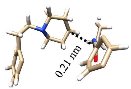
state -2 (higher energy state)
