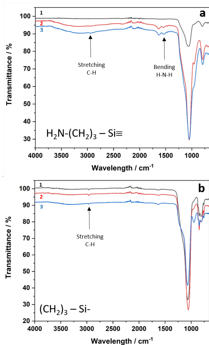
Figure S1.- FTIR spectra of silica supports functionalized with (a) APTES and (b) ClSiMe 3 . (1) FS, (2) UVM-7 and (3) Ti-UVM-7.
