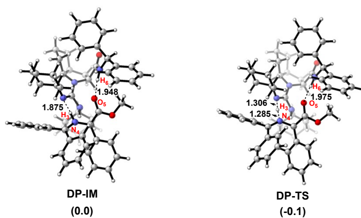
Figure S4 Optimized geometries of intermediate DP-IM and transition state DP-TS in the proton transfer from ylide to the guanidine catalyst G1. The Gibbs free energy of DP-IM was set to zero.
