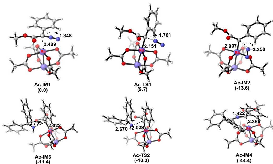
Figure S3 Optimized geometries of transition states in the C-N bond formation step, catalyzed by \text{Rh}_2(\text{OAc})_4 . Relative Gibbs energy was in \text{kcal mol}^{-1} .
