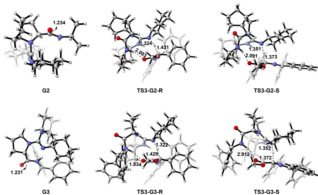
Figure S8 Optimized geometries of transition states in the C-H formation step in the reaction catalyzed by G2 and G3, respectively.
