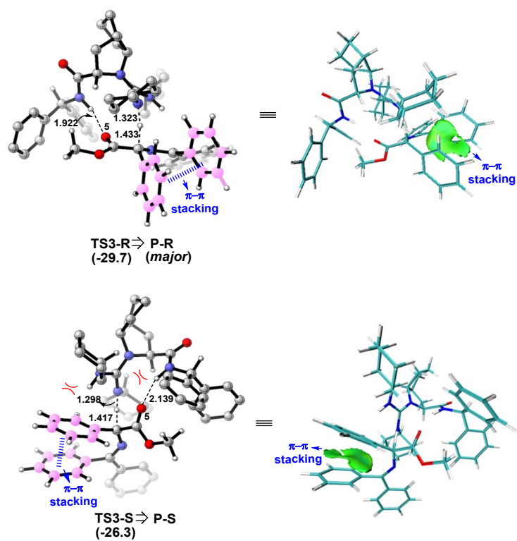
Figure S5 Optimized geometries of transition states TS3-R and TS3-S. the noncovalent analysis was performed by Multiwfn 3.8 (dev).
