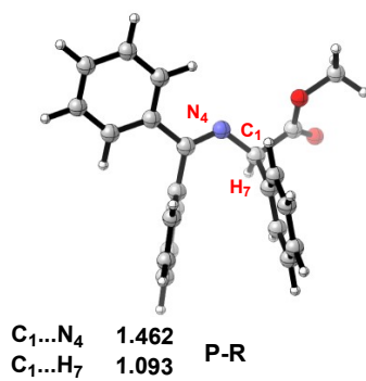
Figure S2 Optimized geometries of intermediates and transition states in the catalytic reaction.
