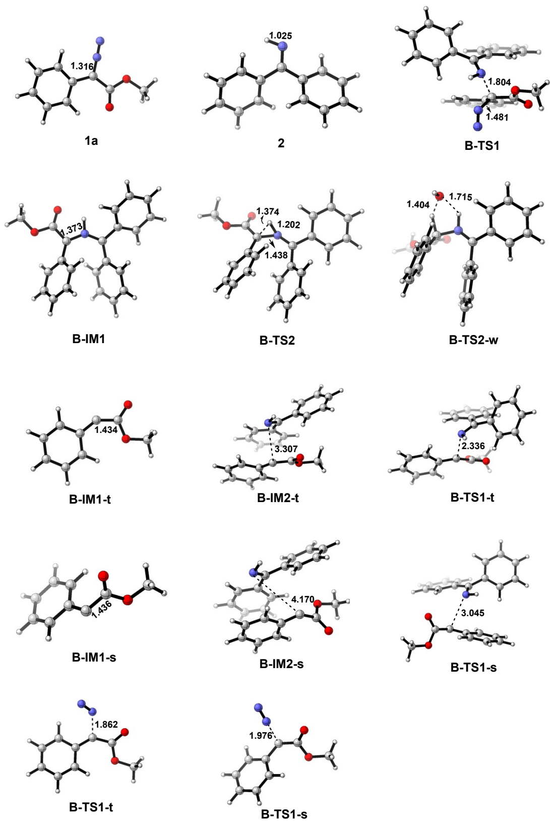
Figure S1 Optimized geometries of intermediates and transition states in the non-catalytic reaction.
