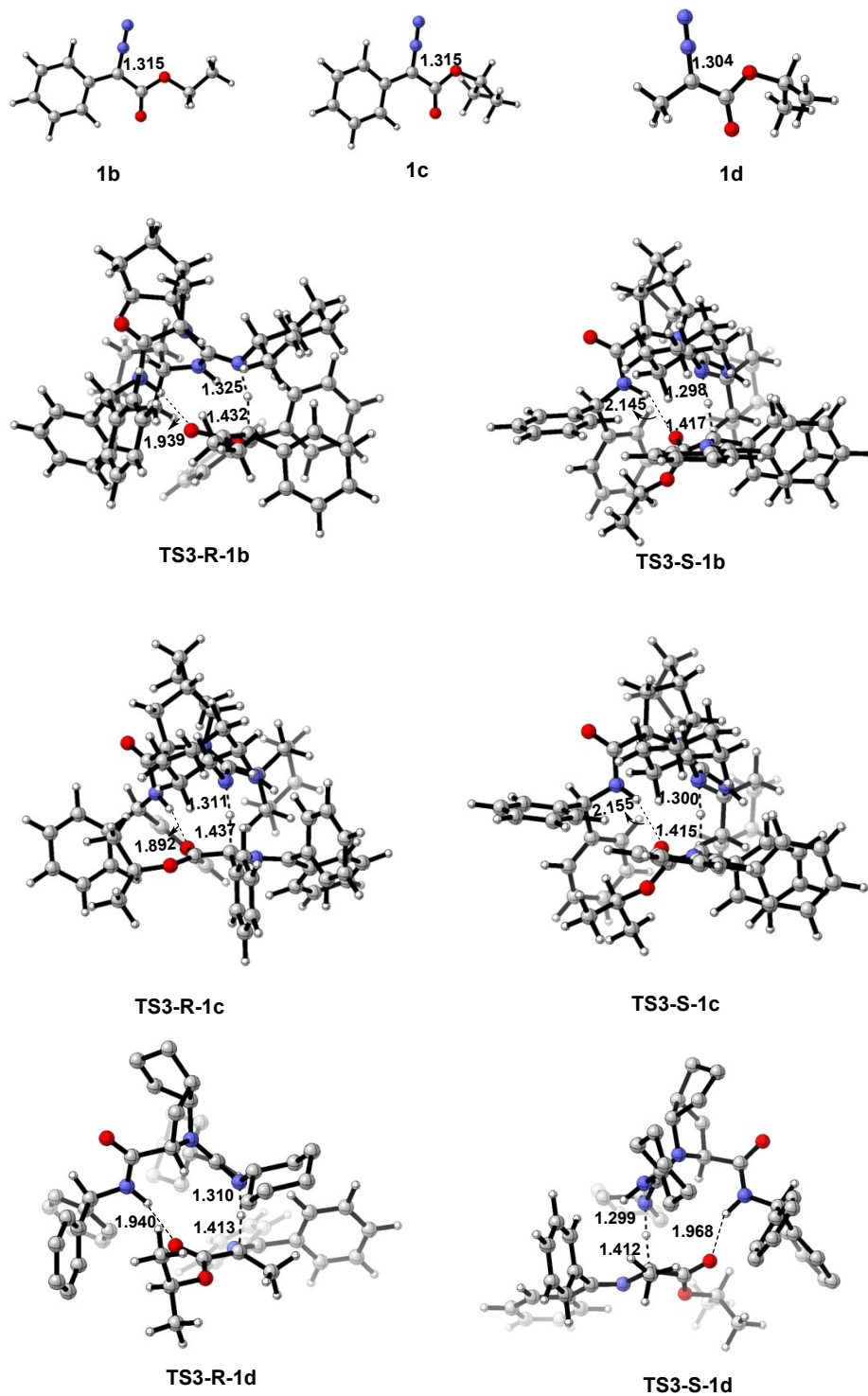
Figure S6 Optimized geometries of transition states in the C-H formation step in the catalytic reactions using 1b~1d as substrates.
