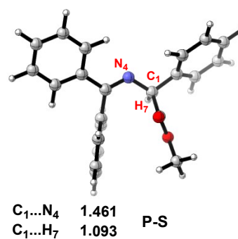
Figure S2 Optimized geometries of intermediates and transition states in the catalytic reaction.
