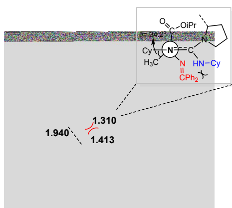
Figure S7 Optimized geometries of transition states of TS3-R, TS3-S, TS3-R-1d and TS3-S-1d.
