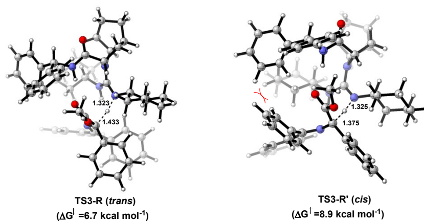
Figure S9 The optimized geometries of TS3-R and TS3-R', with the CPh 2 moiety of the enolate ion oriented either trans or cis to the COOMe group, respectively.
