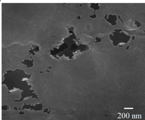
Fig. 2: FESEM images of dried PP film at different magnifications
