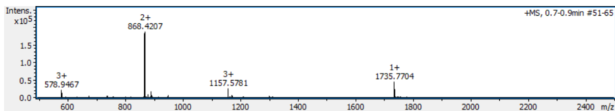
Figure S29. Analytical HPLC trace and ESI MS for product 49 ; analytical gradient 10-80% B over 10 min, 210 nm. Calculated Mass [M+H] + : 1734.82, [M+2H] 2+ : 867.91. Observed Mass [M+H] + : 1735.77, [M+2H] 2+ : 868.42.
