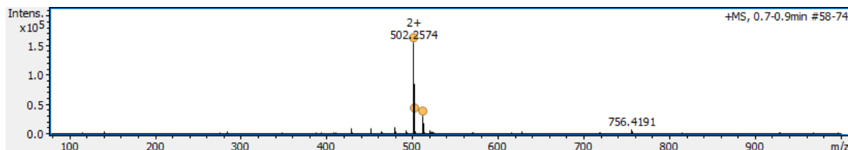
Figure S30. Analytical HPLC trace and ESI MS for product 51 ; analytical gradient 10-30% B over 10 min, 210 nm. Calculated mass [M+2H]^{2+} : 502.25; observed mass [M+2H]^{2+} : 502.26.
