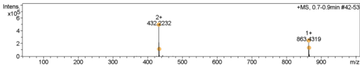
Figure S23 - Analytical HPLC trace and ESI MS for product 33 ; analytical gradient 5-60% B over 10 min, 210 nm. Calculated mass [M+H] + : 863.42; observed mass [M+H] + : 863.43.
