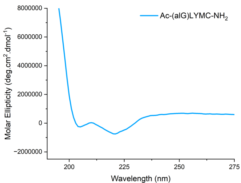
Figure S84. Circular dichroism of cyclised product 23a .
