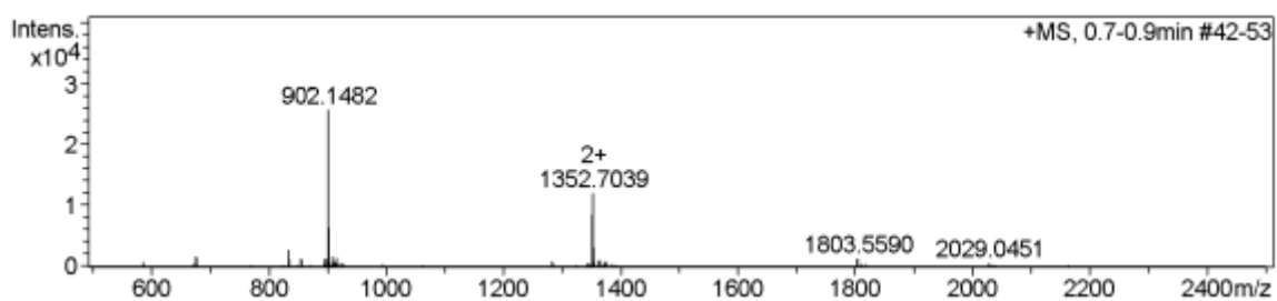
Figure S34. Analytical HPLC trace and ESI MS for product 56 ; analytical gradient 30-100% B over 10 min, 280 nm. Calculated mass [M+2H]^{2+} : 1352.20; observed mass [M+2H]^{2+} : 1352.70.
