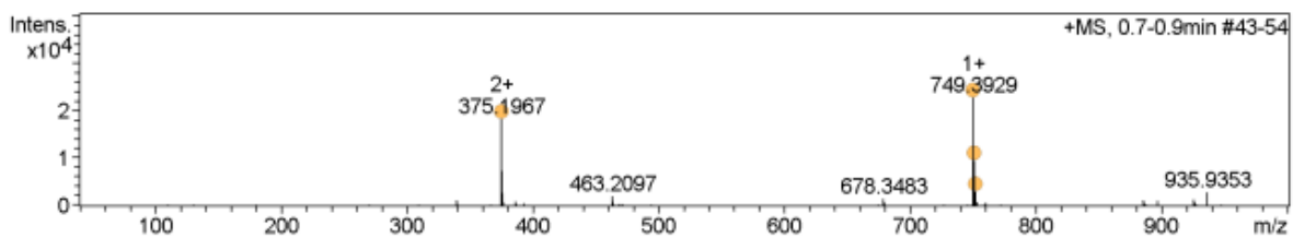
Figure S112. Analytical HPLC trace and ESI MS of purified cyclisation of Ac-(aIG)RPMHC-NH 2 ( 40b ); analytical gradient 2-95% B over 10 minutes, 210 nm. Calculated mass [M+H] + : 749.38; observed mass [M+H] + 749.39.
