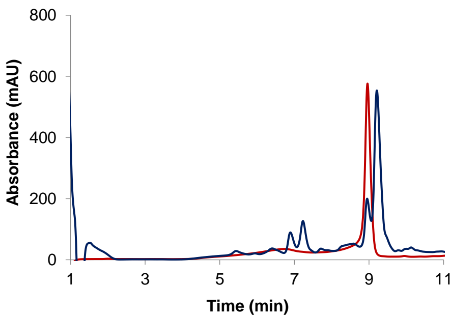
Figure S43. Crude analytical HPLC (blue) trace of cyclised H-(alG)AFAC-NH 2 ( 8a ); analytical gradient 2-25% B over 10 minutes, 210 nm. Red trace – H-(alG)AFAA-NH 2 ( 9 ).
