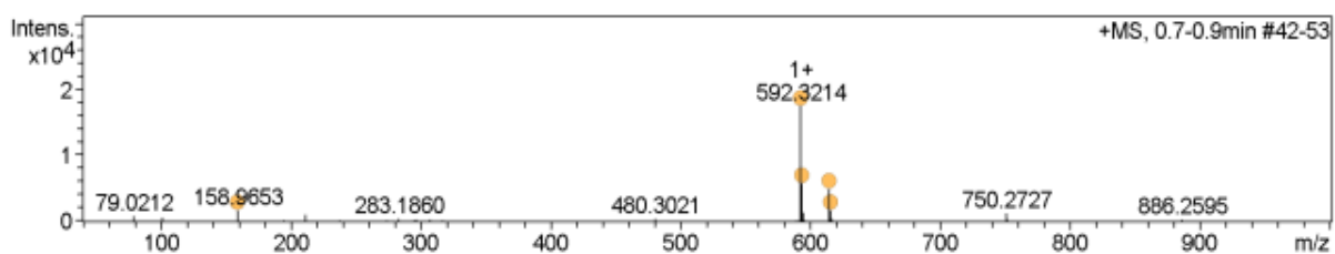
Figure S89. Analytical HPLC trace and ESI MS of purified cyclisation of Ac-(aIG)VHQC- NH 2 ( 24 ); analytical gradient 2-95% B over 10 minutes, 210 nm. Calculated mass [M+H] + : 592.31; observed mass [M+H] + : 592.32.
