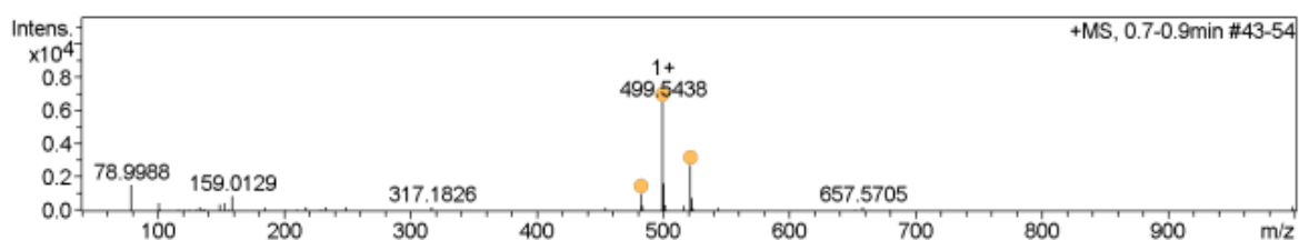
Figure S95. Analytical HPLC trace and ESI MS of purified cyclisation of Ac-(aIG)VGDC-NH 2 ( 26 ); analytical gradient 2-70% B over 10 minutes, 210 nm. Calculated mass [M+H] + : 499.24; observed mass [M+H] + 499.54.
