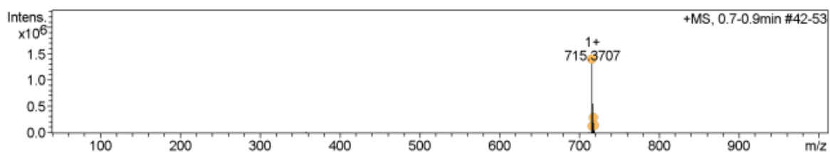
Figure S10 - Analytical HPLC trace and ESI MS for product 15 ; analytical gradient 15-80% B over 10 min, 210 nm. Calculated mass [M+H] + : 715.36; observed mass [M+H] + : 715.37.
