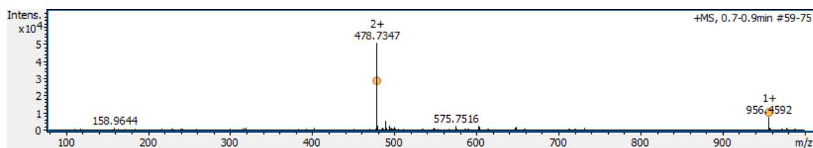
Figure S139. Analytical HPLC trace and ESI MS of cyclised H-(aI G )DKFNHEC-NH 2 ( 47 ); analytical gradient 2-25% B over 10 minutes, 210 nm. Calculated mass [M+H] + : 956.45, [M+2H] 2+ : 478.73; observed mass [M+H] + : 956.46, [M+2H] 2+ : 478.73.
