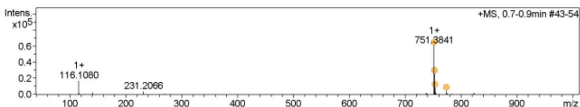
Figure S17 - Analytical HPLC trace and ESI MS for product 28 ; analytical gradient 15-80% B over 10 min, 280 nm. Calculated mass [M+H] + : 751.37; observed mass [M+H] + : 751.38.
