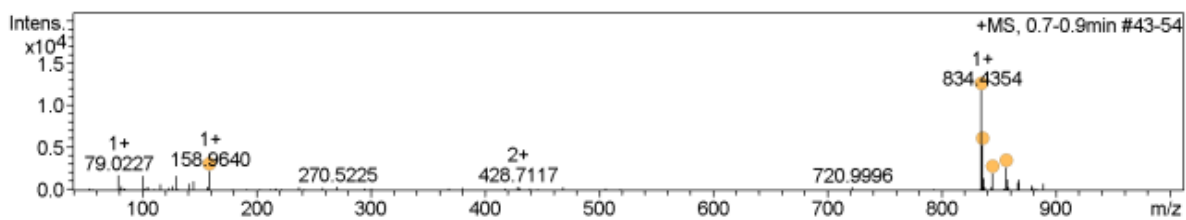
Figure S122. Analytical HPLC trace and ESI MS of purified cyclisation of Ac-(aIG)DSYKIC-NH 2 ( 42 ); analytical gradient 5-60% B over 10 minutes, 210 nm. Calculated mass [M+H] + : 834.43; observed mass [M+H] + 834.44.
