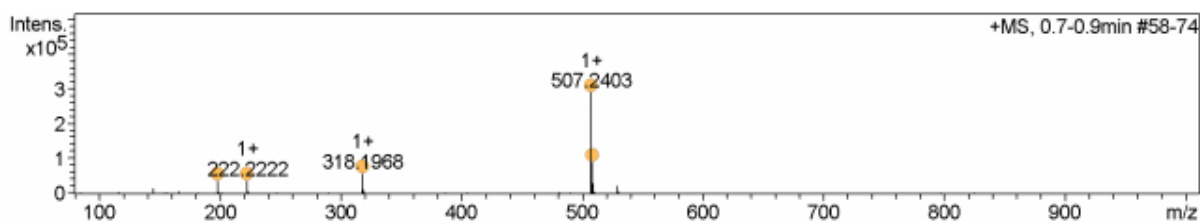
Figure S4. Analytical HPLC trace and ESI MS for product 7a ; analytical gradient 10-30% B over 10 min, 210 nm. Calculated mass [M+H]^+ : 507.23; observed mass [M+H]^+ : 507.24.
