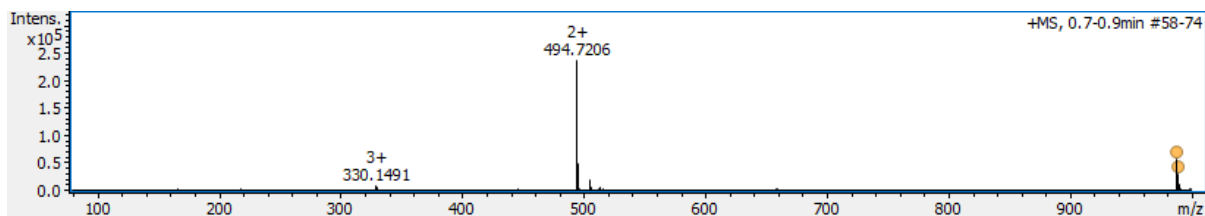
Figure S27. Analytical HPLC trace and ESI MS for product 37 ; analytical gradient 2-25% B over 10 min, 210 nm. Calculated mass [M+2H]^{2+} : 494.71; observed mass [M+2H]^{2+} : 494.72.
