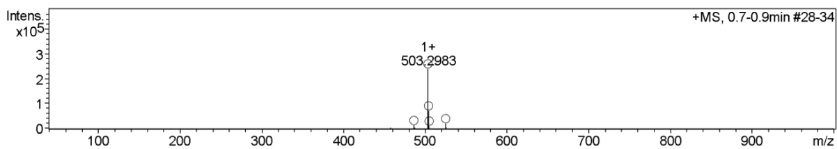
Figure S70. Analytical HPLC trace and ESI MS of purified cyclisation of H-(pG)AFAC-NH 2 ( 11 ); analytical gradient 5-40% B over 10 minutes, 280 nm. Calculated mass [M+H] + : 503.29; observed mass [M+H] + : 503.30.
