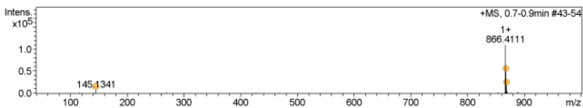
Figure S22 - Analytical HPLC trace and ESI MS for product 32 ; analytical gradient 5-60% B over 10 min, 210 nm. Calculated mass [M+H] + : 866.40; observed mass [M+H] + : 866.41.
