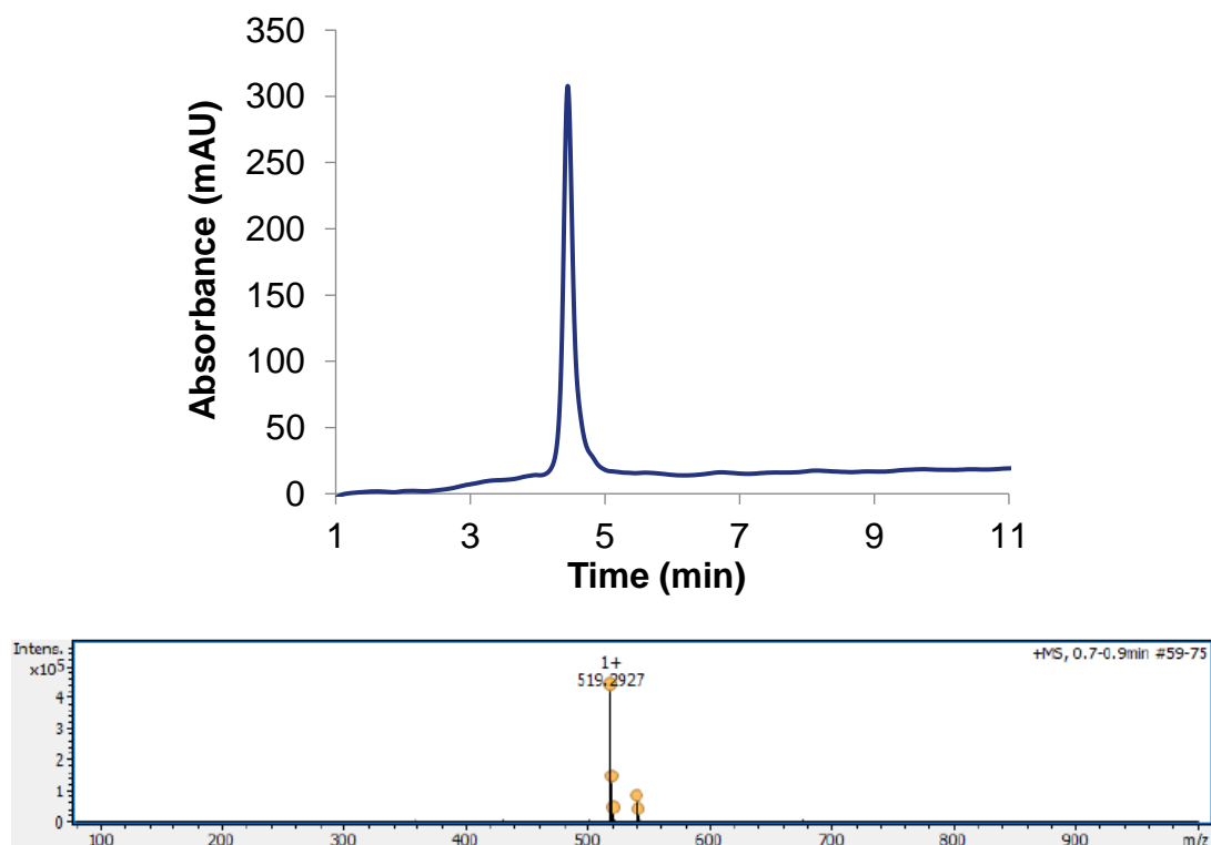
Figure S37. Analytical HPLC trace and ESI MS of purified diastereomer A from the cyclisation of H-S(OAllyl)AFAC-NH 2 ; analytical gradient 10-30% B over 10 minutes, 210 nm. Calculated mass [\text{M}+\text{H}]^+ : 519.29; observed mass [\text{M}+\text{H}]^+ : 519.29.
