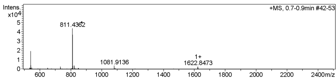
Figure S33. Analytical HPLC trace and ESI MS for product 55 ; analytical gradient 2-95% B over 5 min, 210 nm. Calculated mass [M+H] + : 1621.85; observed mass [M+H] + : 1622.85.
