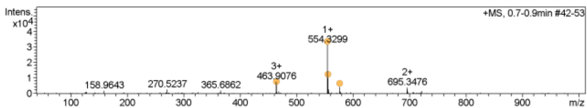
Figure S92. Analytical HPLC trace and ESI MS of purified cyclisation of Ac-(aIG)TPKC-NH 2 ( 25 ); analytical gradient 5-60% B over 10 minutes, 210 nm. Calculated mass [M+H] + : 554.32; observed mass [M+H] + : 554.33.
