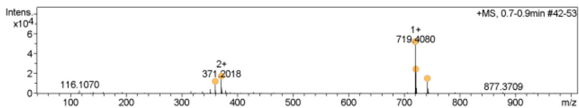
Figure S101. Analytical HPLC trace and ESI MS of purified cyclisation of Ac-(aIG)KISYC-NH 2 ( 39 ); analytical gradient 5-60% B over 10 minutes, 210 nm. Calculated mass [M+H] + : 719.40; observed mass [M+H] + 719.41.
