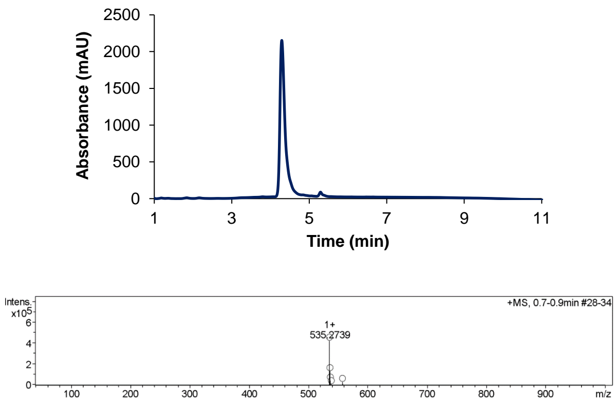
Figure S7 - Analytical HPLC trace and ESI MS for product 10 ; analytical gradient 15-80% B over 10 min, 210 nm. Calculated mass [M+H] + : 535.26; observed mass [M+H] + : 535.27
