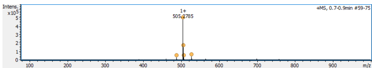
Figure S41. Analytical HPLC trace and ESI MS of cyclised H-S(OAllyl)AFAC-NH 2 ( 6 ); analytical gradient 2-25% B over 10 minutes, 210 nm. Calculated mass [M+H] + : 505.27; observed mass [M+H] + : 505.28.
