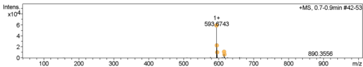
Figure S86. Analytical HPLC trace and ESI MS of purified cyclisation of H-(aIG)LYMC-NH 2 ( 23b ); analytical gradient 15-80% B over 10 minutes, 210 nm. Calculated mass [M+H] + : 593.30; observed mass [M+H] + : 593.67.
