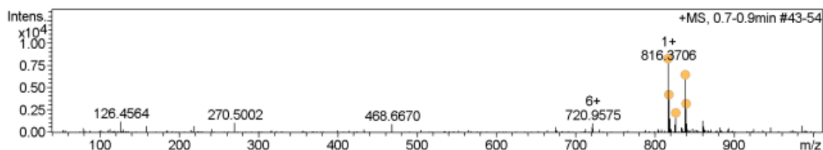
Figure S21 - Analytical HPLC trace and ESI MS for product 31 ; analytical gradient 2-95% B over 10 min, 210 nm. Calculated mass [M+H] + : 816.36; observed mass [M+H] + : 816.37.
