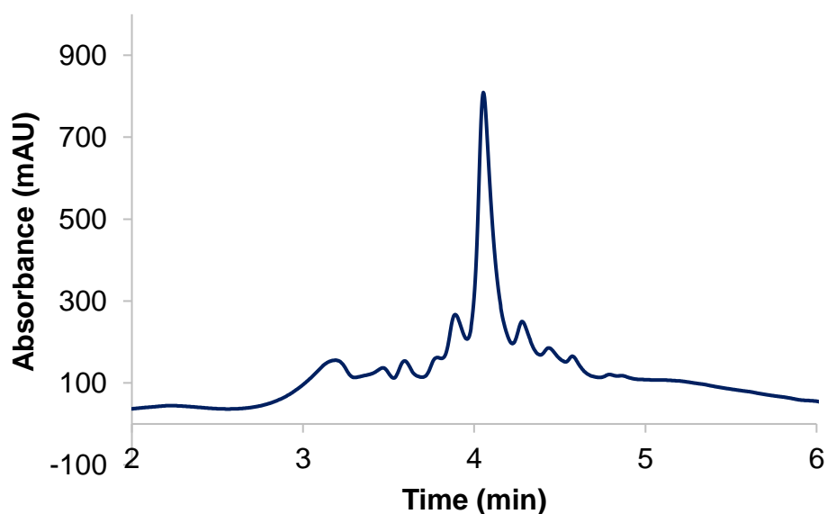
Figure S141. Crude analytical HPLC trace of Ac-(aIG)QVGDSN L C-NH 2 ( 48 ) cyclisation; analytical gradient 2-95% B over 5 minutes, 210 nm.
