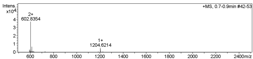
Figure S151. Analytical HPLC trace and ESI MS of cyclised Ac-HLA(aIG)VGDCN L DR-NH 2 ( 57 ); analytical gradient 2-95% B over 5 minutes, 210 nm. Calculated mass [M+H] + : 1204.64; observed mass [M+H] + : 1204.62.
