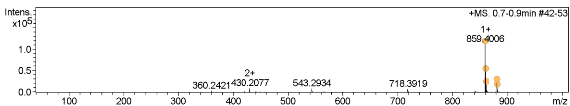
Figure S28. Analytical HPLC trace and ESI MS for product 38 ; analytical gradient 2-95% B over 5 min, 210 nm. Calculated mass [M+H] + : 859.39; observed mass [M+H] + : 859.40.
