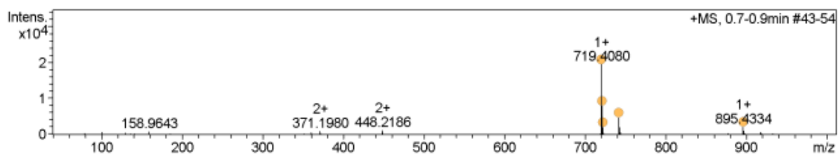
Figure S109. Analytical HPLC trace and ESI MS of purified cyclisation of Ac-CKISY(alG)-NH 2 ( 39 ); analytical gradient 2-95% B over 10 minutes, 210 nm. Calculated mass [M+H] + : 719.41; observed mass [M+H] + 719.40.
