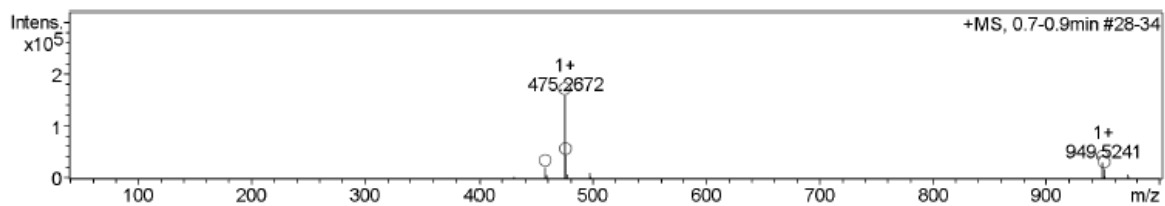
Figure S60. Analytical HPLC trace and ESI MS of desired product ( 8a ) isolated at 21.5 min; analytical gradient 2-25% B over 10 minutes, 210 nm.
