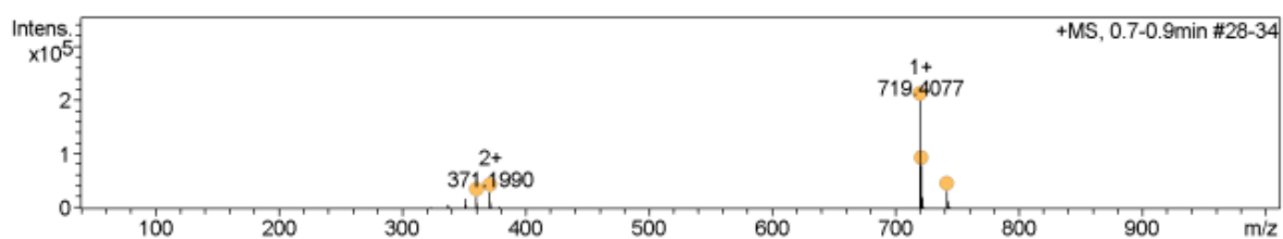
Figure S105. Analytical HPLC trace and ESI MS of purified cyclised product 39 ; analytical gradient 5-60% B over 10 minutes, 280 nm. Calculated mass [M+H]^+ : 719.40; observed mass [M+H]^+ 719.41.
