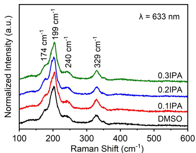
Figure S1 Raman spectra of the CZTSSe thin films fabricated from precursor solutions with varying IPA ratios.
