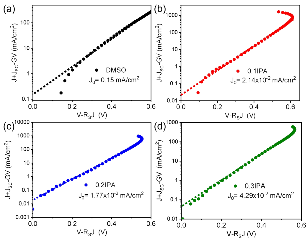
Figure S2 The plots of J + J_{SC} - GV versus V - R_s J .
