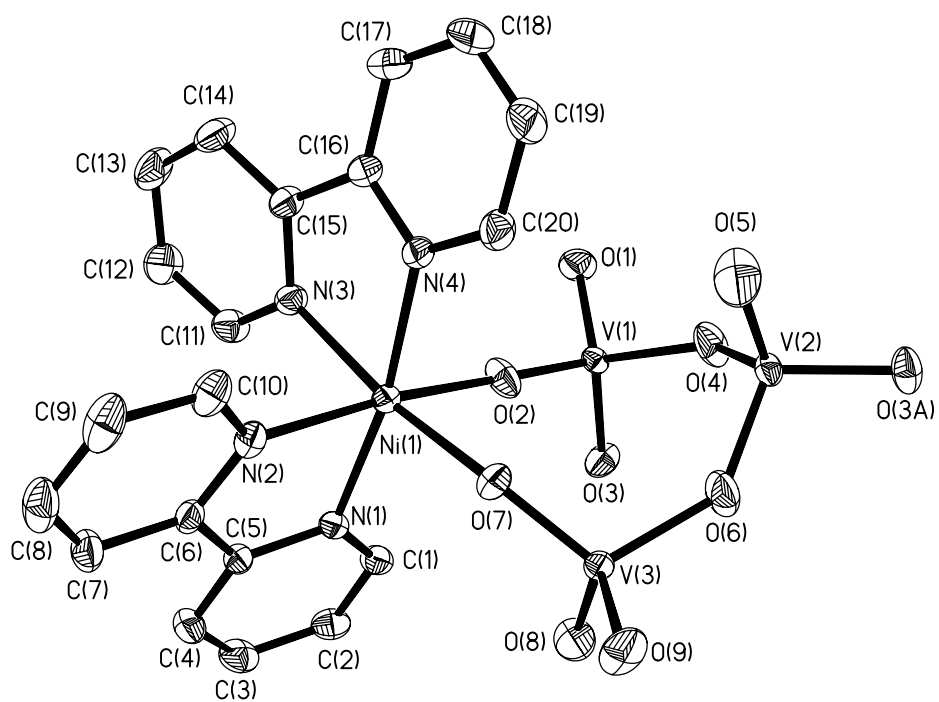
Fig. S3. A basic structure unit of the layer with the atomic labeling scheme (30% probability) in complex 2 .
