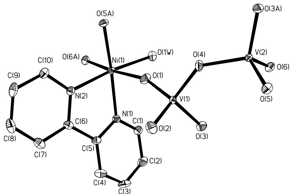
Fig. S1. A fragment of the net with the atomic labeling scheme (30% probability) in complex 1.
