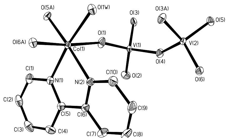
Fig. S2. A fragment of the net with the atomic labeling scheme (30% probability) in complex 3.
