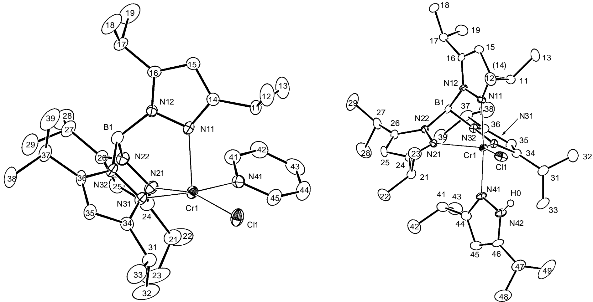
Figure S1. Atomic numbering schemes for 1b (left) and 1a (right). Labels without atom names are for carbon atoms.
