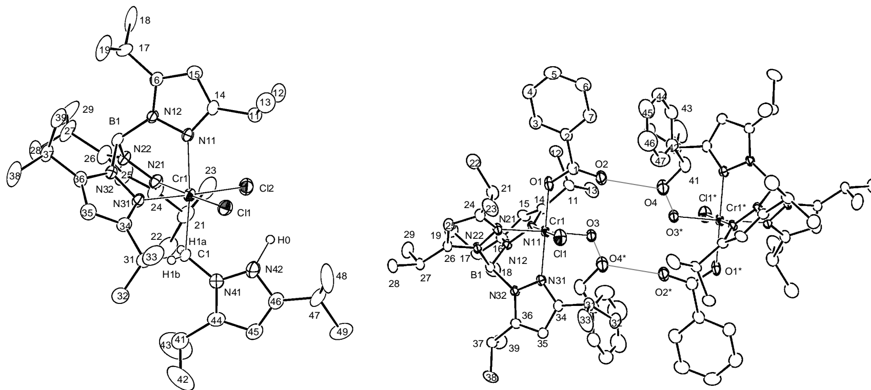
Figure S4. Atomic numbering schemes for the 7a (left) and 9 (right). Labels without atom names are for carbon atoms.
