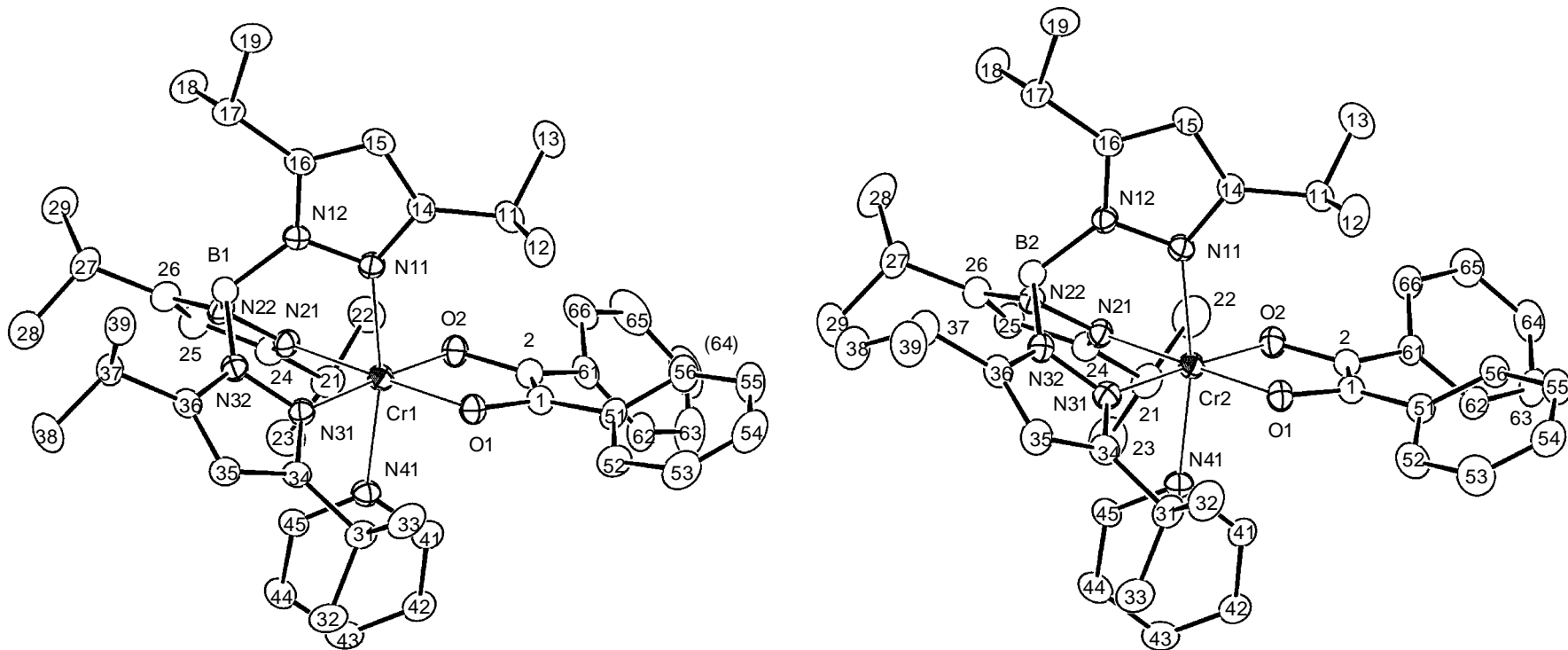
Figure S5. Atomic numbering schemes for the 8 (left: A-series; right B-series). Labels without atom names are for carbon atoms.
