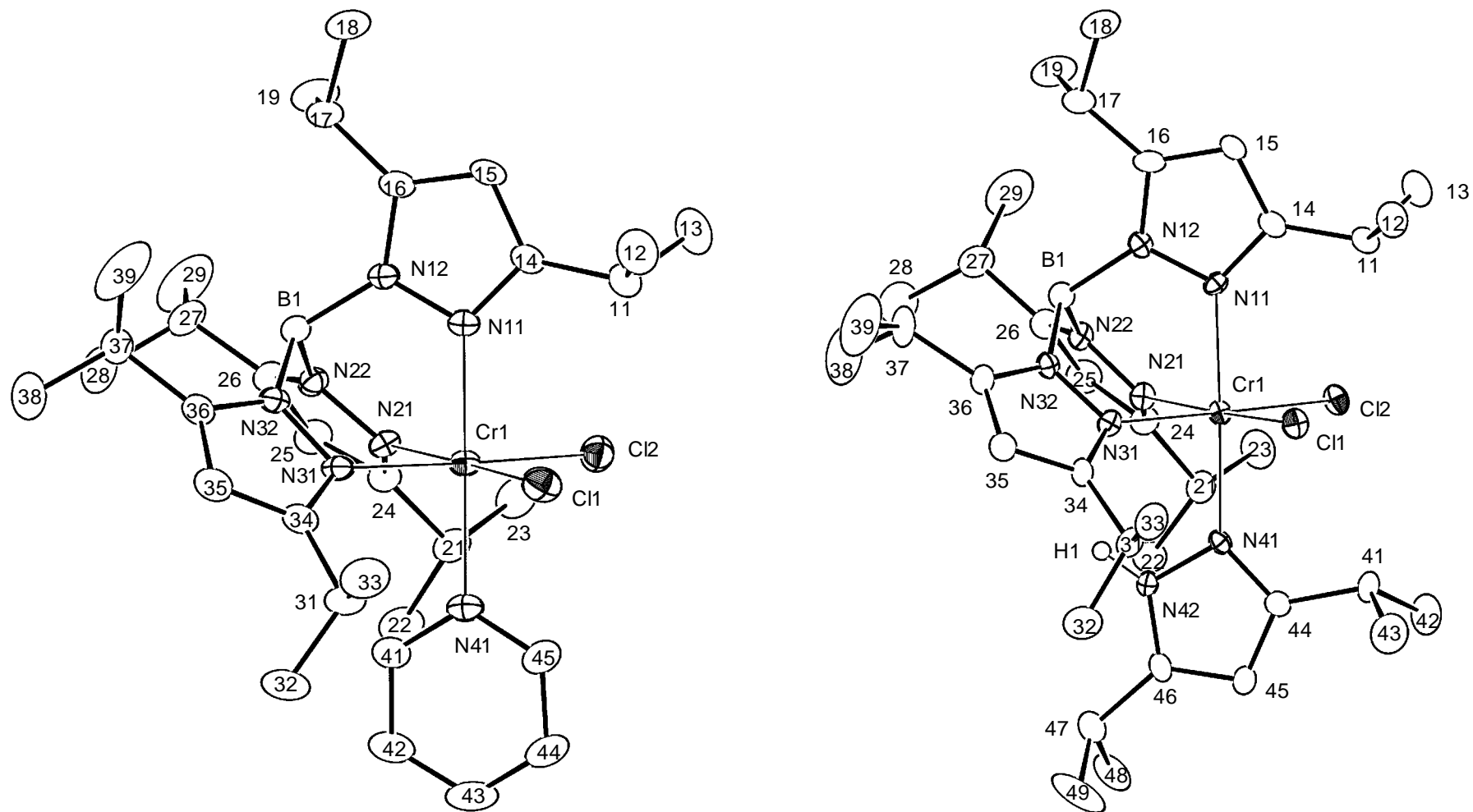
Figure S3. Atomic numbering schemes for 6b . (left) and 6a (right). Labels without atom names are for carbon atoms.
