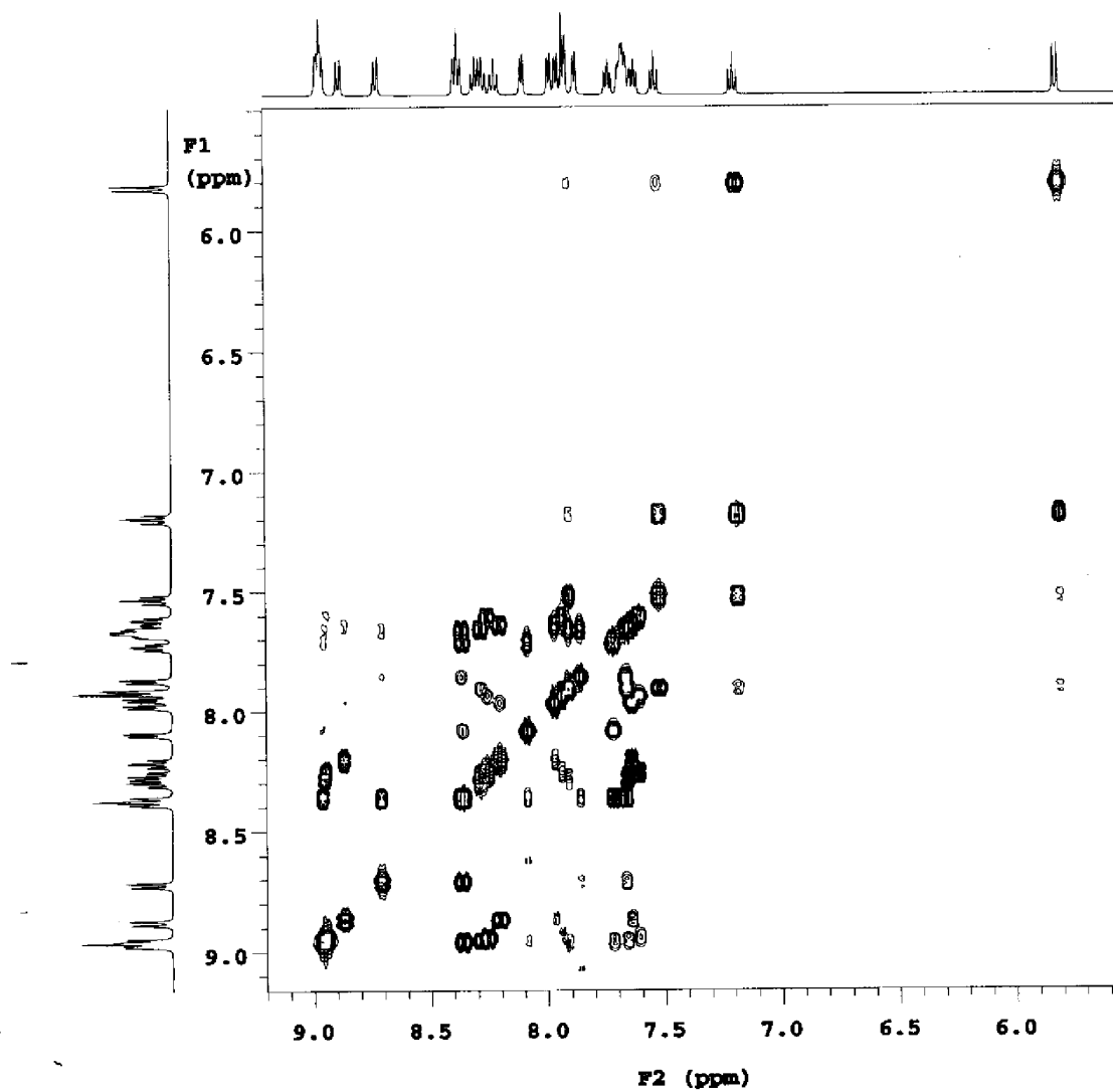
Fig. S1 ^1\text{H} - ^1\text{H} COSY of [(\text{bpy})_2\text{Ru}(\text{pbimH})](\text{PF}_6)_2 in MeCN
