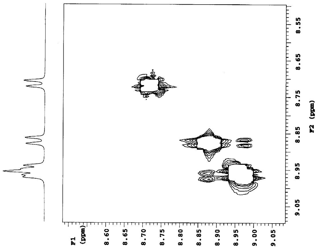
Fig. S2 ^1\text{H} - ^1\text{H} NOESY of [(\text{bpy})_2\text{Ru}(\text{pbimH})](\text{PF}_6)_2 in MeCN
