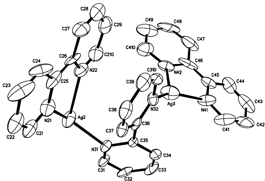
Fig. S1 Thermal ellipsoid plot of [\text{Ag}_2(2, 2'\text{-bipy})_3]^{2+} groups showing the coordination environment around Ag(2) and Ag(3) and their connectivity.
