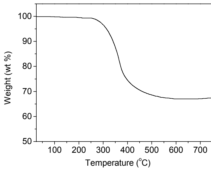
Fig. S4 The TG curve of compound 1
