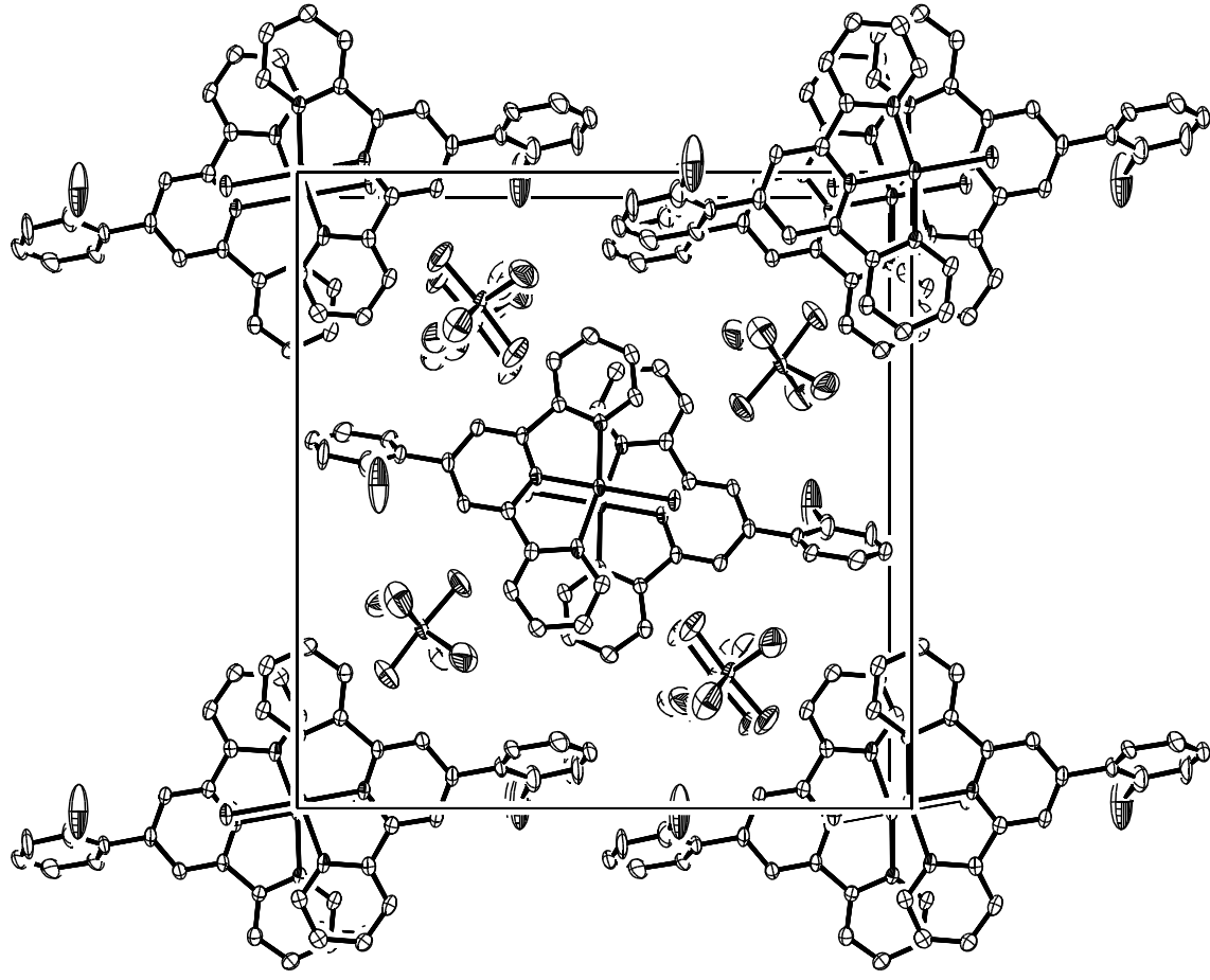
Fig. S1. View down the [a]-axis of the unit cell of [Pt{4'-(o-Cl-Ph)trpy}Cl]SbF 6
