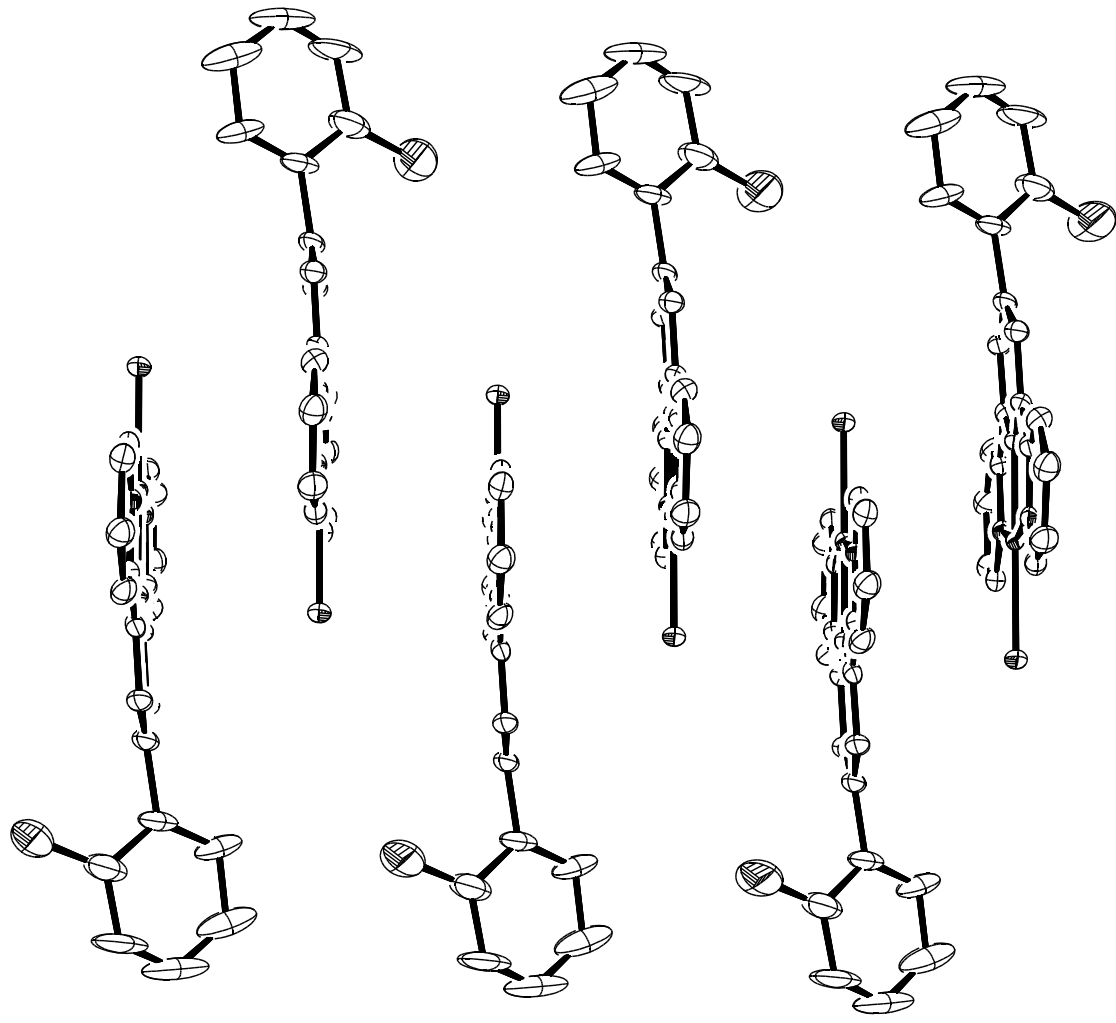
Fig. S2. View of the cation stack in [\text{Pt}\{4'-(o\text{-Cl-Ph})\text{trpy}\}\text{Cl}]\text{SbF}_6
