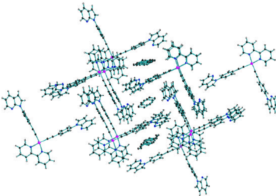
Figure 5. Unit cell packing diagram showing the location of solvent molecules in the crystal lattice of 1 .
