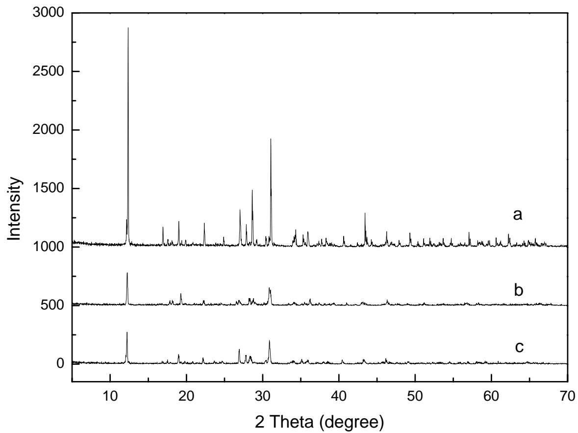
XRD patterns of (a) \text{KGaTeO}_5 \cdot \text{H}_2\text{O} ; (b) \text{Na}^+ -exchanged \text{KGaTeO}_5 \cdot \text{H}_2\text{O} ; (c) \text{Rb}^+ -exchanged \text{KGaTeO}_5 \cdot \text{H}_2\text{O}
