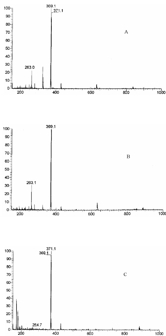
Figure S1. ESI-MS spectra for complexes 1 (A), \text{AgCF}_3\text{SO}_3\text{-L}^1 (B), and \text{AgPF}_6\text{-L}^1 (C)
