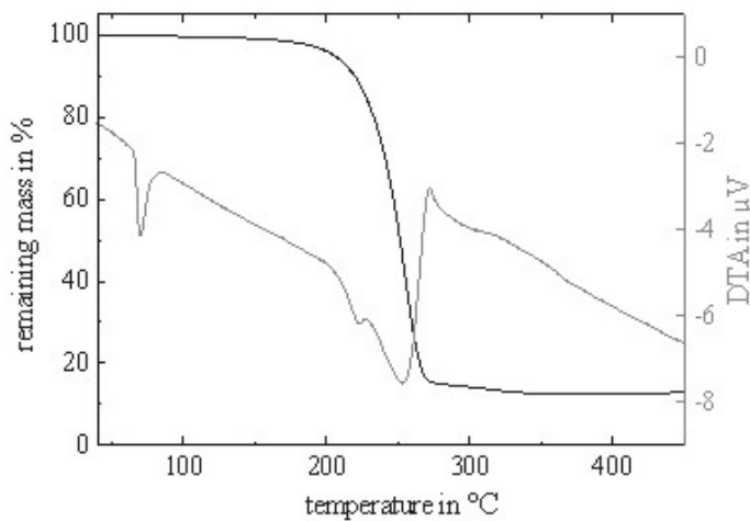
TG/DTA – spectrum of Compound 2 (Heating Rate 5°C/min, N 2 -flow 300ml min -1 )
