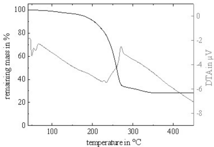
TG/DTA – spectrum of Compound 1 (Heating Rate 5°C/min, N 2 -flow 300ml min -1 )
