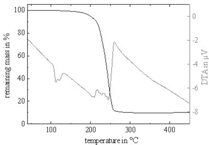
TG/DTA – spectrum of Compound 3 (Heating Rate 5°C/min, N 2 -flow 300ml min -1 )
