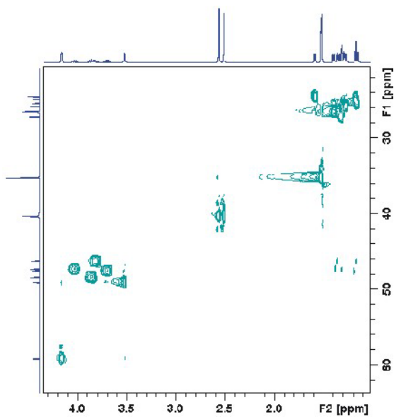
2-D HMQC – spectrum of Compound 1 (C 6 D 6 , RT)
