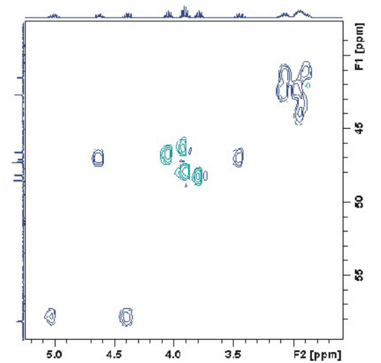
2-D HMQC – spectrum of Compound 3 (C 6 D 6 , RT)
