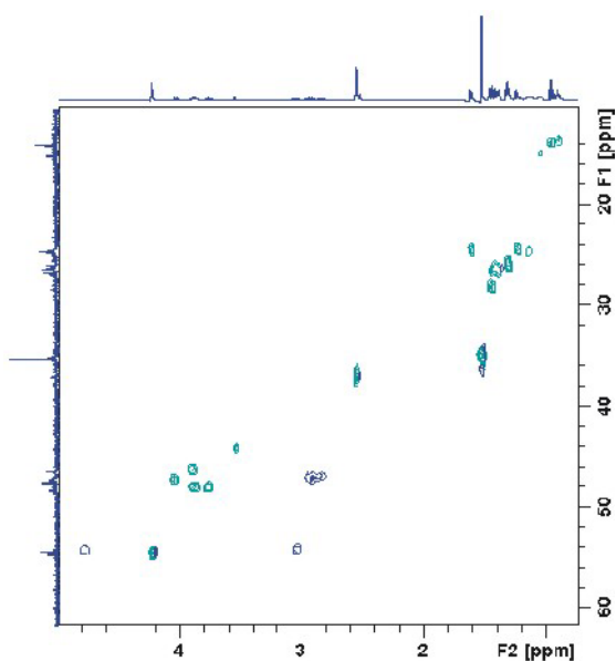
2-D HMQC – spectrum of Compound 2 (C 6 D 6 , RT)
