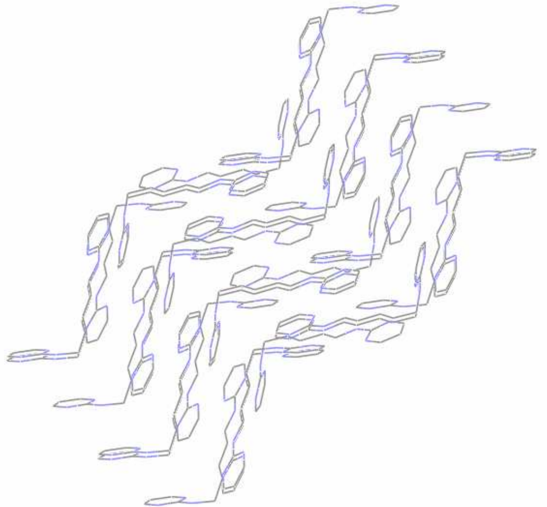
Figure 5. Crystal packing of pyr 2 C 5 IV
