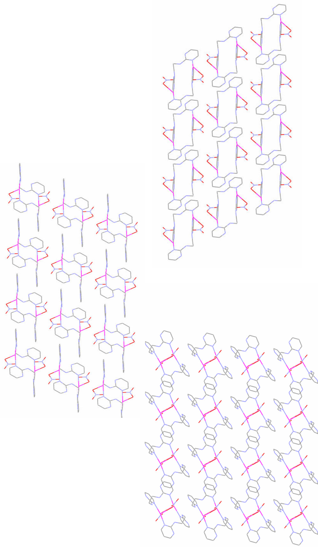
Figure 7. Crystal packing of Pyr 2 C 2 -Ag complex 1 (views along a , b , c axis, respectively)
