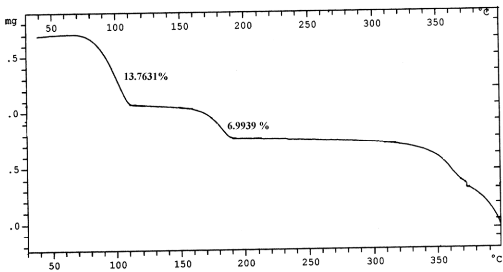
Fig. S2. TG curve of complex 3.
