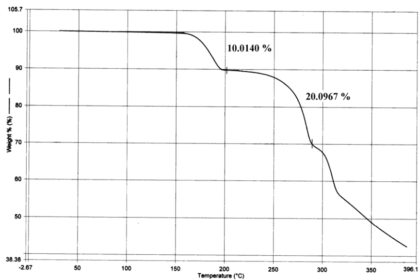
Fig. S1. TG curve of complex 2.
