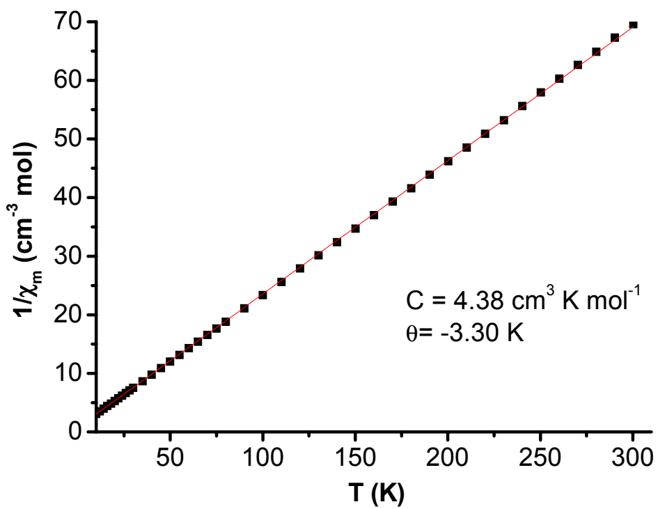
Fig. S2 Inverse of the molar magnetic susceptibility of 1 vs temperature.
