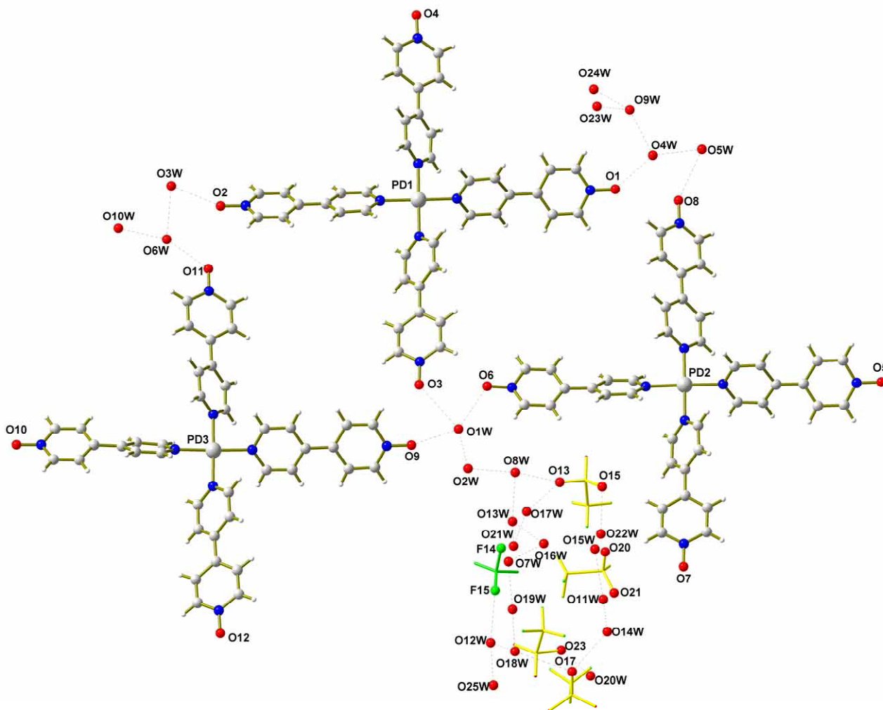
Figure S-2: Full packing arrangement of in-plane cations, anions and water molecules for [\text{Pd}(\text{BIPYMO})_4]_3[\text{OTf}]_4[\text{BF}_4]_2
