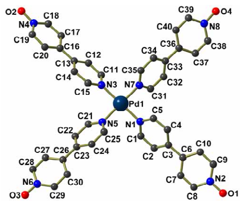
Figure S-1: [\text{Pd}(\text{BIPYMO})_4]_3[\text{OTf}]_4[\text{BF}_4]_2
