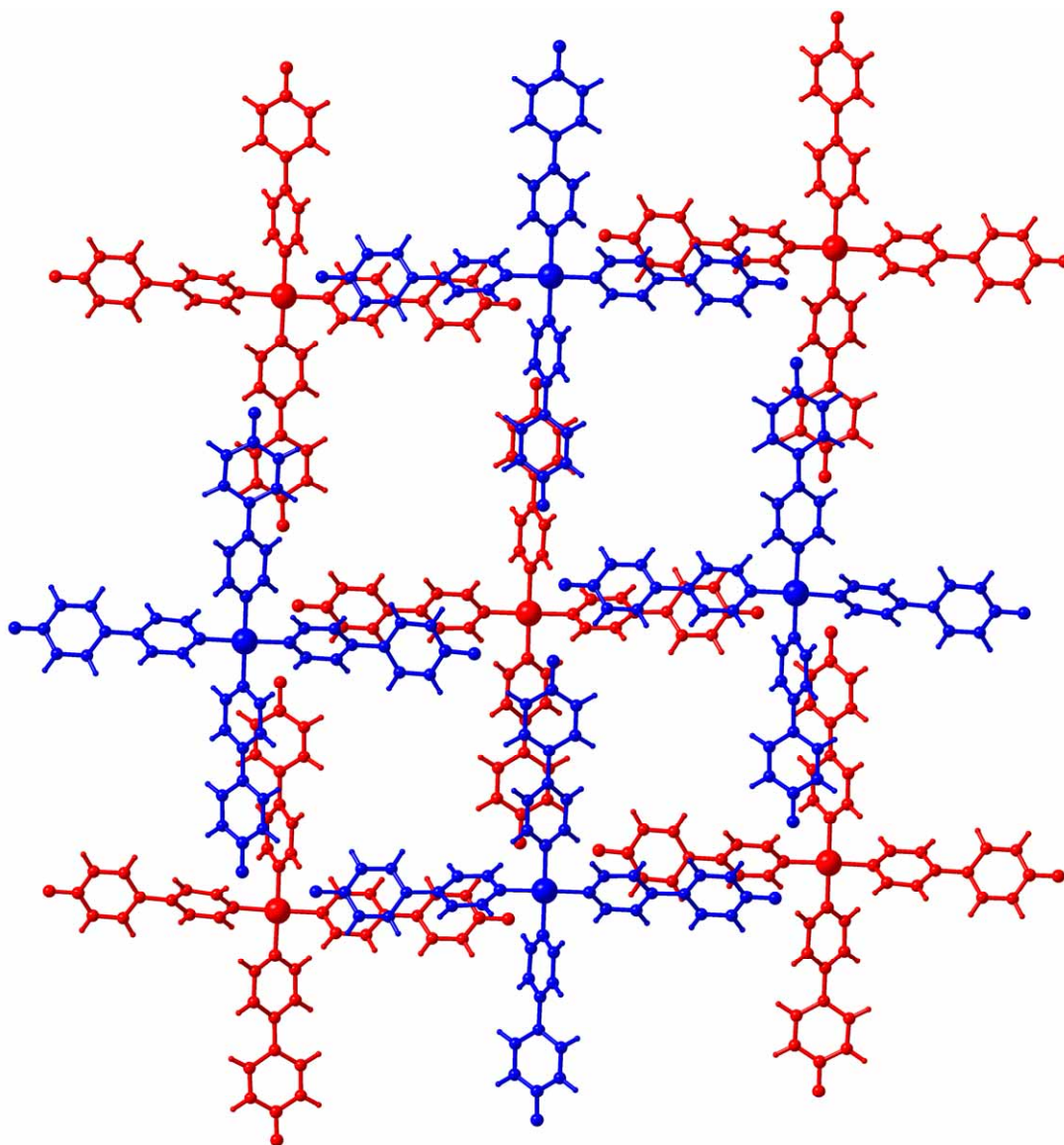
Figure S-3: A packing diagram for [\text{Pd}(\text{BIPYMO})_4]_3[\text{OTf}]_4[\text{BF}_4]_2 showing how two layers (red and blue molecules) are organized with respect to each other.
