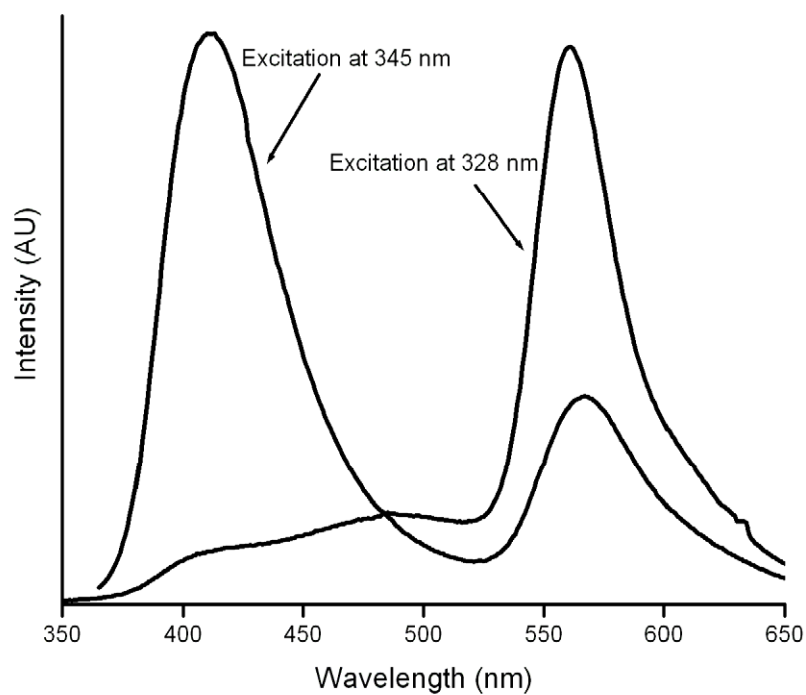
Fig. 2 Emission spectra of 1 in CH 2 Cl 2 . Excitations were performed at 345 nm and 328 nm.
