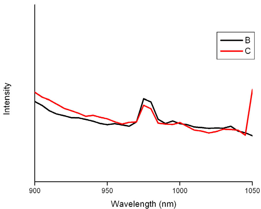
Figure 3. Emission spectra of Yb1 without (Data set 'B') and with added DNA (1 equiv., Data set 'C'). [Yb1] = 0.033 mM, \lambda_{\text{exc}} = 355 nm.
