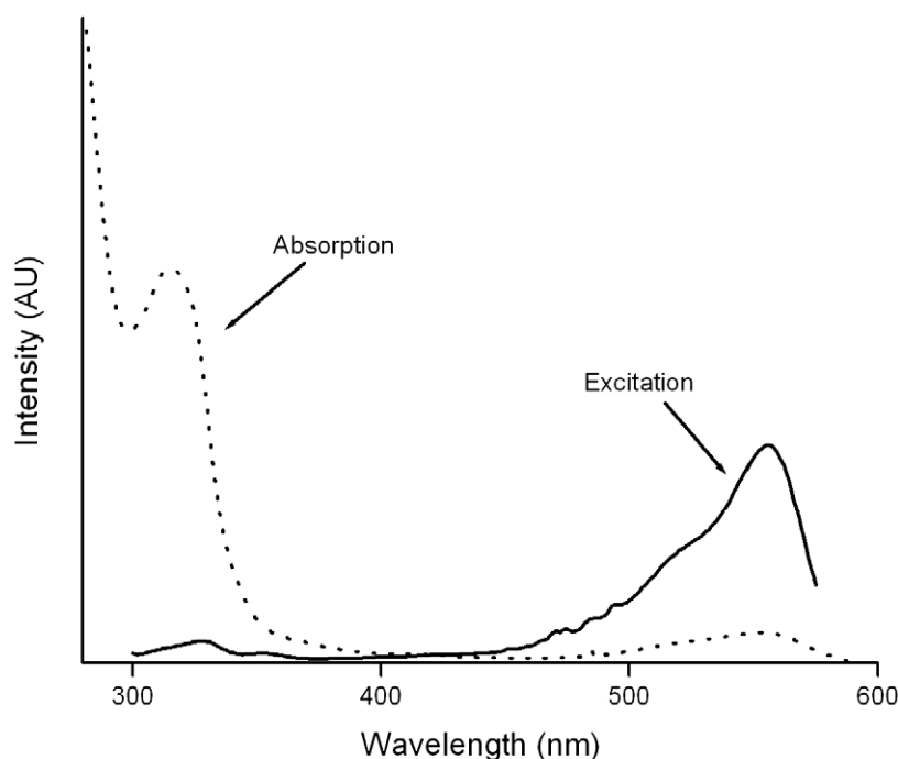
Figure 1. Absorption and excitation spectra of 1 in CH 2 Cl 2 .
