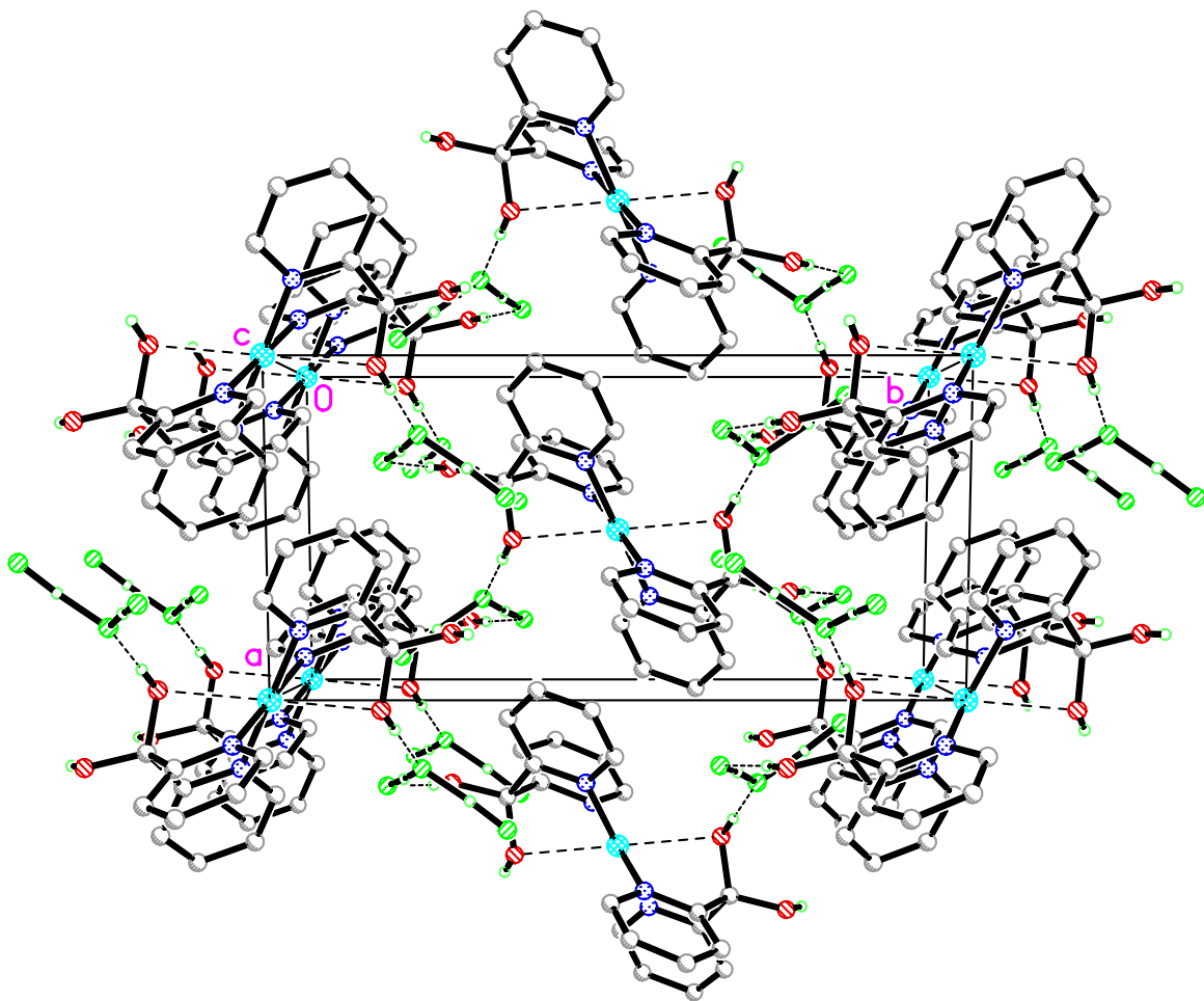
Crystal packing diagram for [Cu(dpdp) 2 ][H 2 F 3 ] 2 viewed along the crystallographic c -axis.
