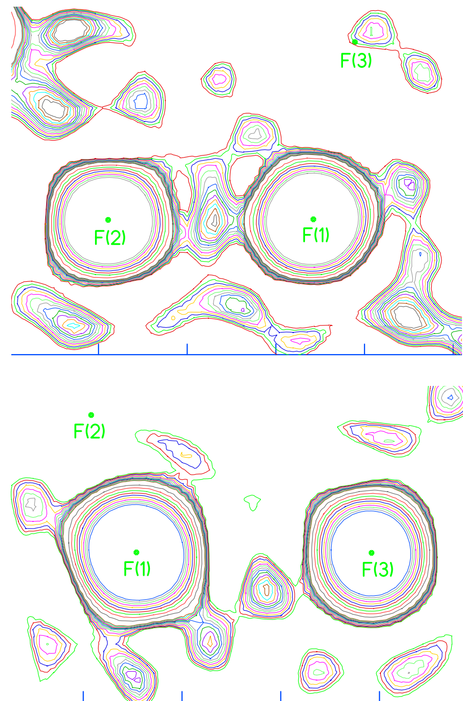
Residual electron density maps for (top) the \text{F}(1)\cdots\text{F}(2) and (bottom) \text{F}(1)\cdots\text{F}(3) segments of the \text{H}_2\text{F}_3^- anion in [\text{Cu}(\text{dpd})_2][\text{H}_2\text{F}_3]_2 . Hash marks on the horizontal axis are 1-Å increments.
