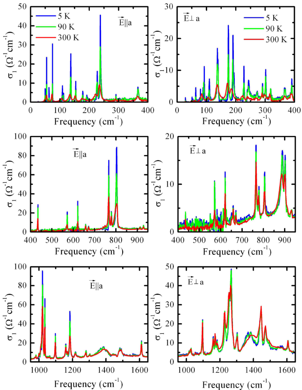
Temperature-dependent and polarized infrared spectra for [\text{Cu}(\text{dpd})_2][\text{H}_2\text{F}_3]_2 .
