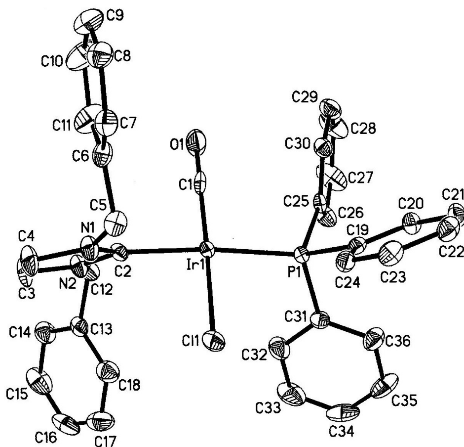
Figure S1. ORTEP plot of 7a
