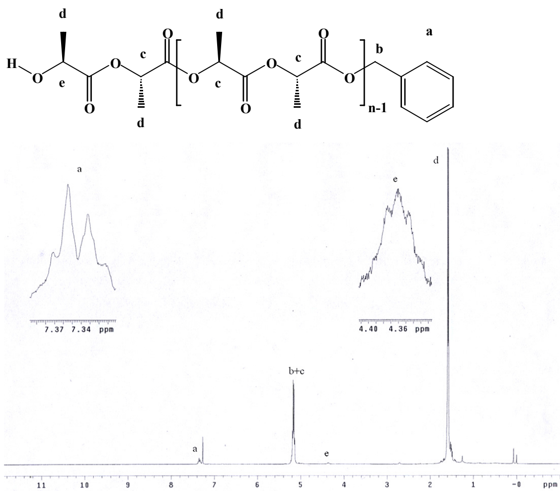
Figure S2. ^1\text{H} NMR spectrum of PLLA-50 in \text{CDCl}_3 .
