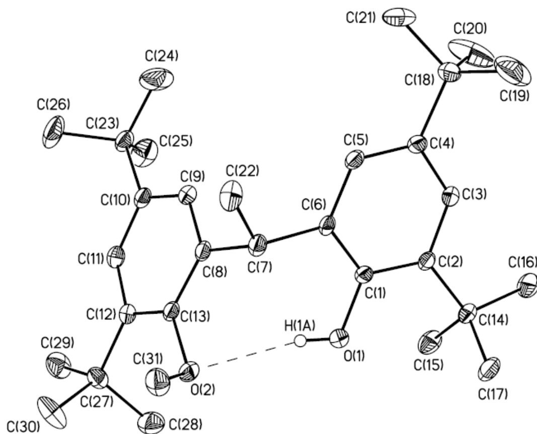
Figure S1. Molecular structure of 1 as 20% ellipsoids, and all of the hydrogen atoms are omitted for clarity.
