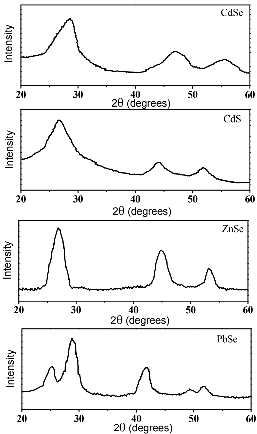
Figure S1: X-ray diffraction patterns of metal chalcogenides nanocrystals
