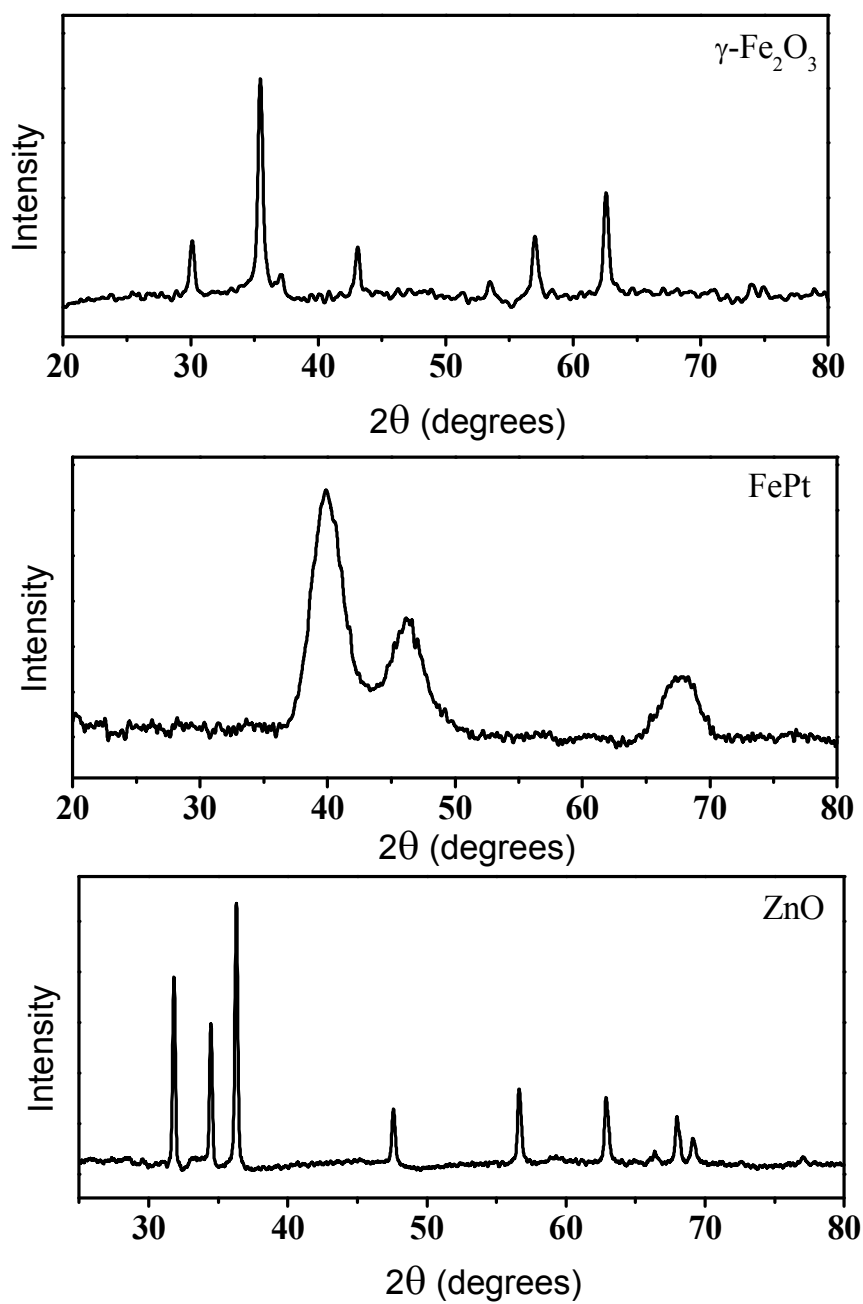
Figure S2: X-ray diffraction patterns of \gamma\text{-Fe}_2\text{O}_3 , FePt and ZnO nanocrystals
