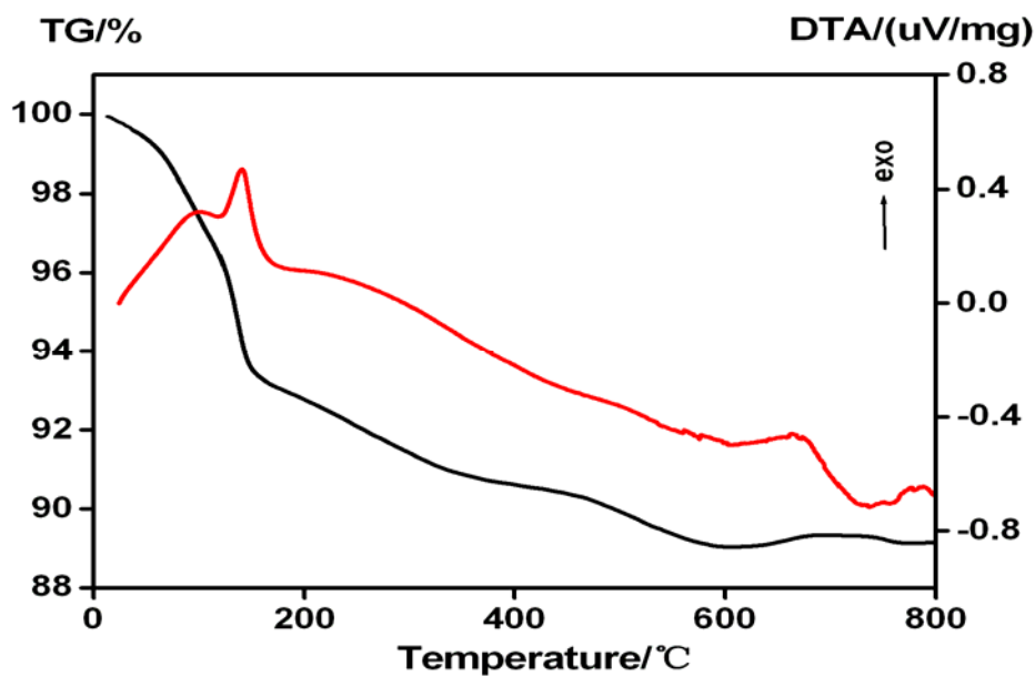
Fig. S2. DSC/TG measurement of compound (1).
