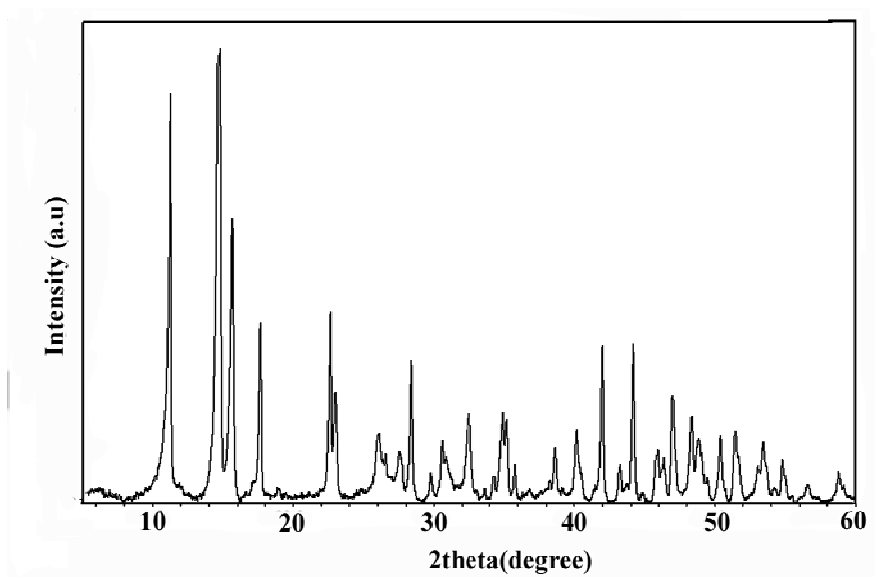
Fig.S1. The X-ray diffraction powder pattern of compound (1).
