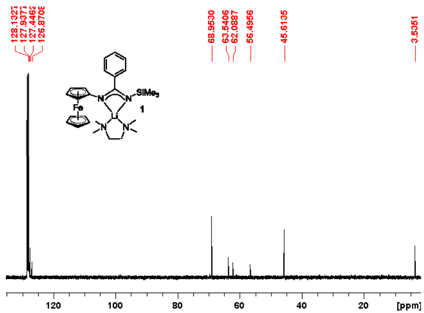
^{13}\text{C} NMR spectrum of compound 1 in \text{C}_6\text{D}_6
