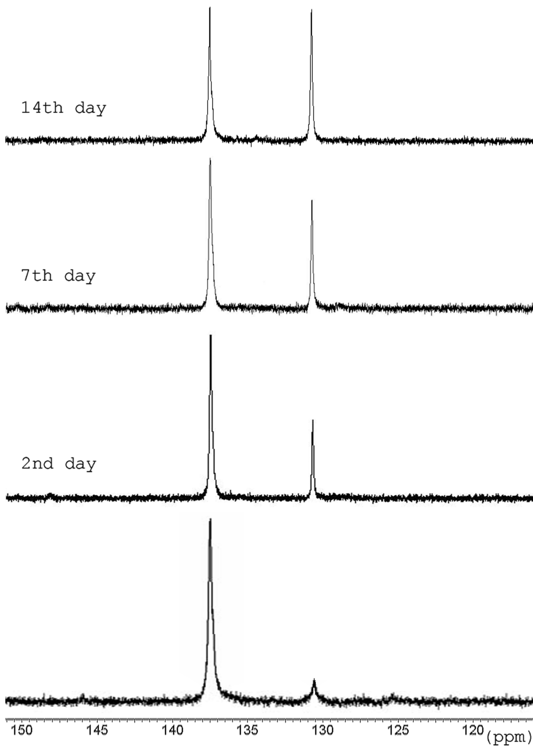
Fig. S1. Dependence of the ^{31}\text{P} NMR spectra in (10) as a function of time.
