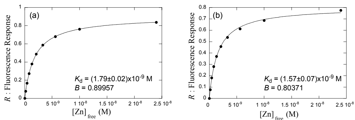
Figure S1. Curve-fitting for calculation of dissociation constants ( K_d ) of (a) 6-MeOBQDIEN and (b) BQDIEN with zinc ion. Experimental data are fitted to equation (1) (see text) using KaleidaGraph software.
