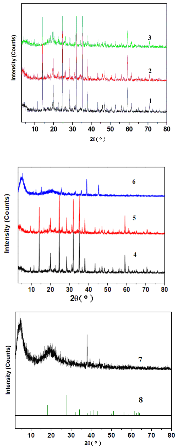
Fig. S2 XRD of ZnPSPPP 1- 7 and 8 ( Zn_3(PO_4)_2 )
