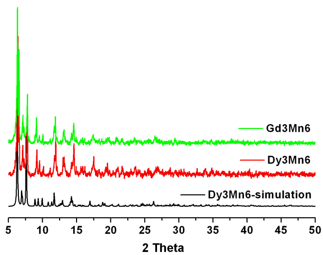
Fig. S3 PXRD patterns of 1 and 3 as-synthesized, together with simulation of 1 according to single crystal structural determinations.
