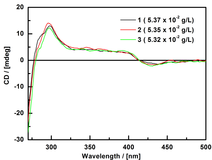
Fig. S2 The CD spectra of bulk samples of 1 , 2 and 3 in methanol.
