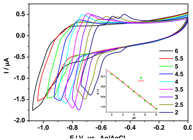
Fig. SI1. CVs of 0.5 mM Eu-GeW 11 using a bare glassy carbon electrode (GCE) as a working electrode at different pHs.
