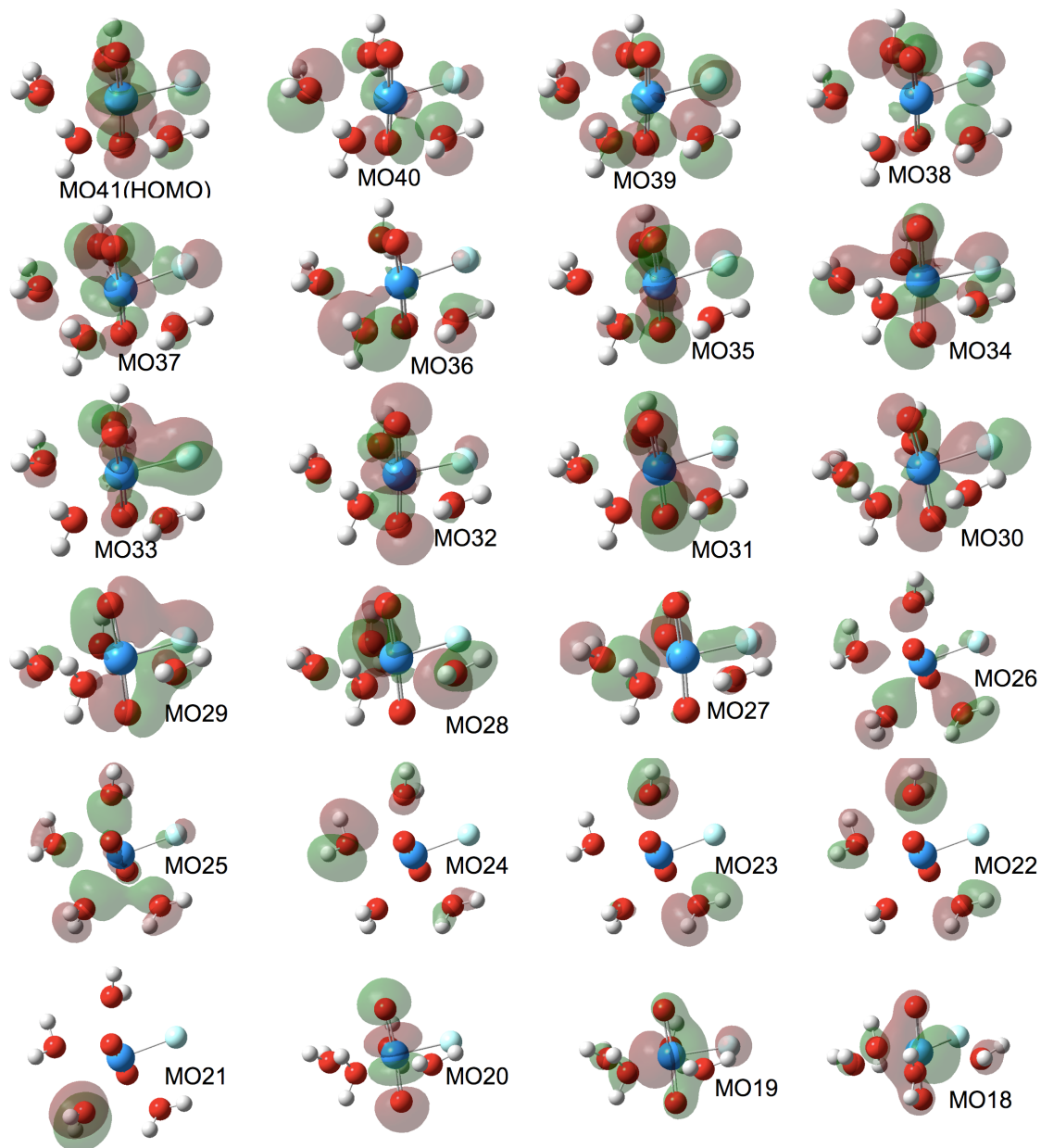
Fig. S2 Molecular orbitals of \text{UO}_2\text{F}^+(\text{aq})
