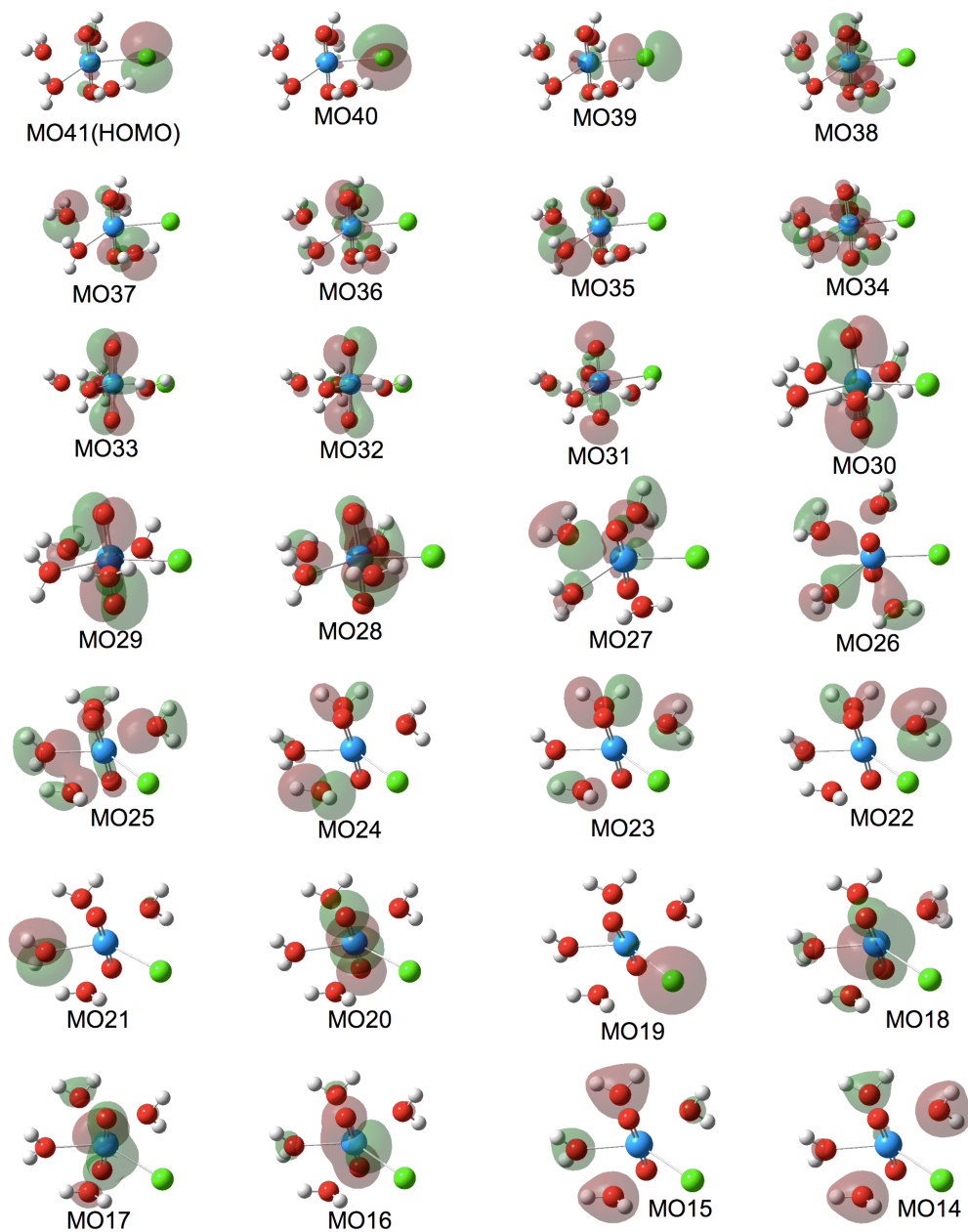
Fig. S1 Molecular orbitals of \text{UO}_2\text{Cl}^+(\text{aq})
