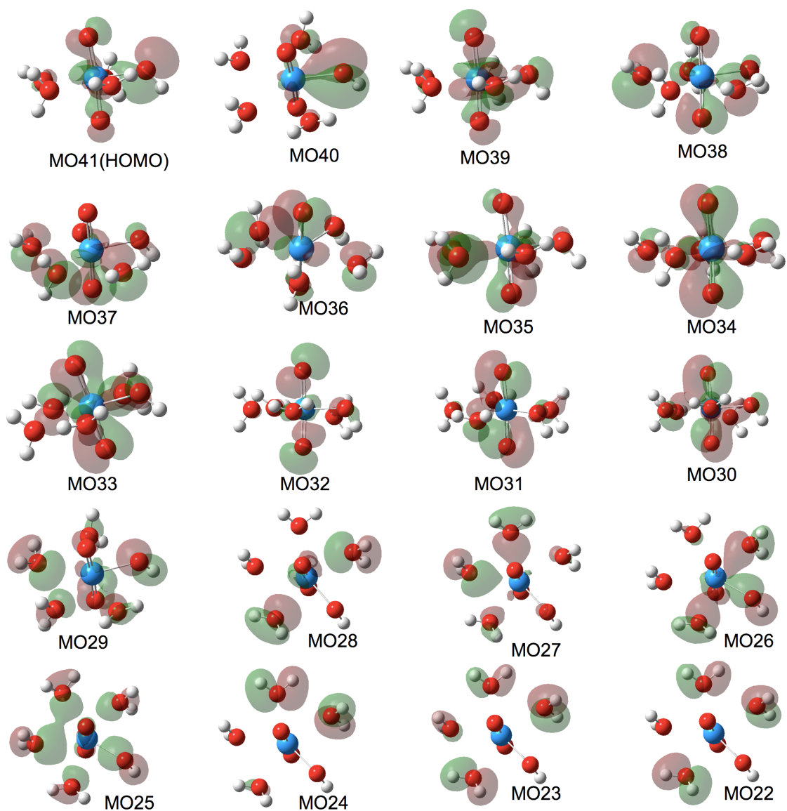
Fig.S3 Molecular orbitals of \text{UO}_2\text{OH}^+(\text{aq})
