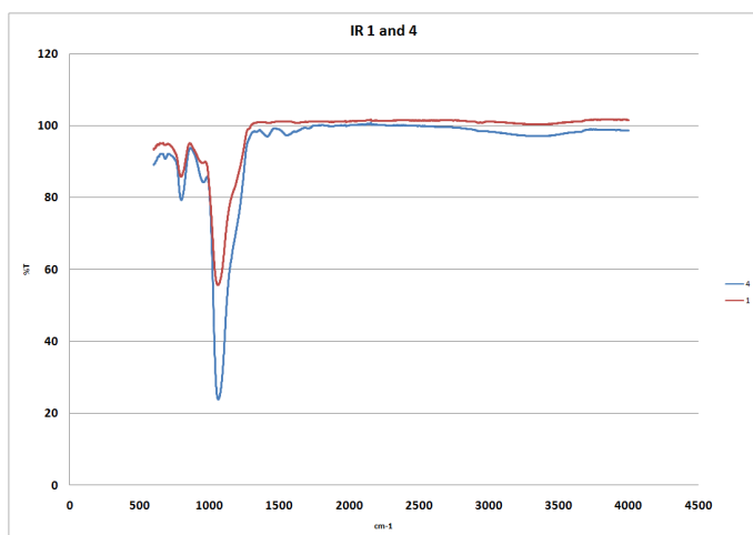
Supplementary Figure A: ATR-IR of 1 and 4
