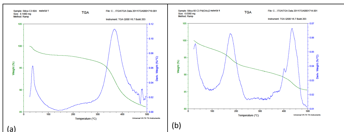
Supplementary Figure B: DTG of 1 (a) 4 (b)
