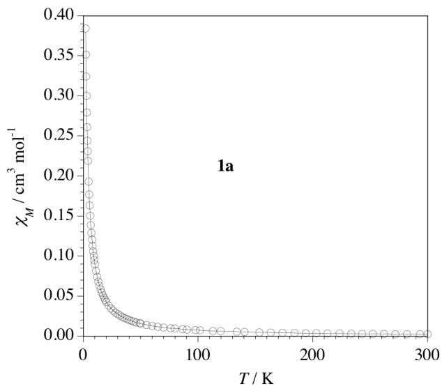
Figure S1. \chi versus T plot for 1a .
