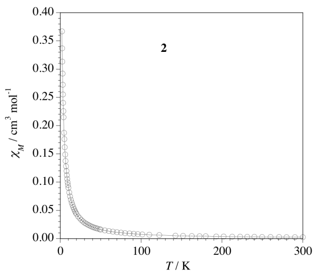
Figure S2. \chi versus T plot for 2 .
