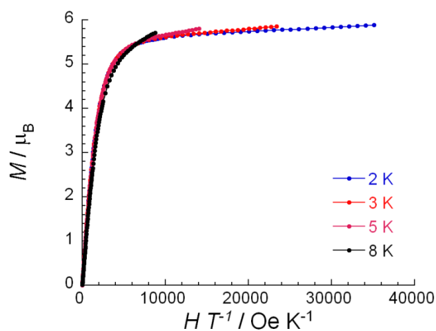
Figure S1. M vs. H/T plot measured between 2 K and 8 K for 1
