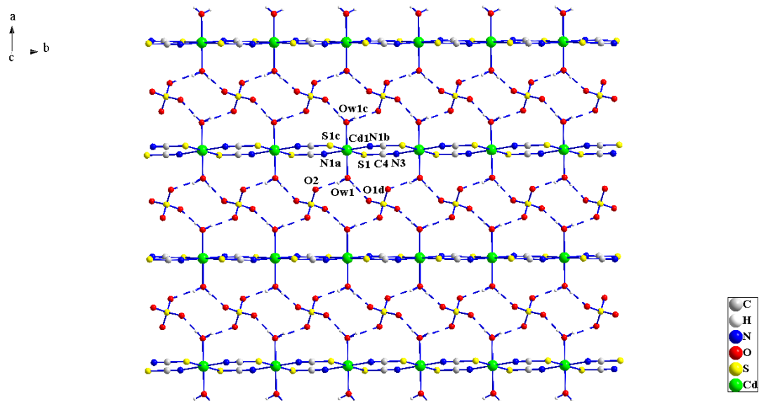
Fig. S1 The 2-D supramolecular network for [\text{Cd}(\text{SCN})_2(\text{H}_2\text{O})_2]\text{SO}_4^{2-} in compound 1 .
