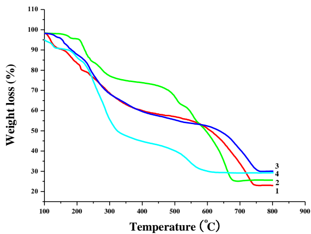
Fig. S3 The TG curves of compounds 1-4.
