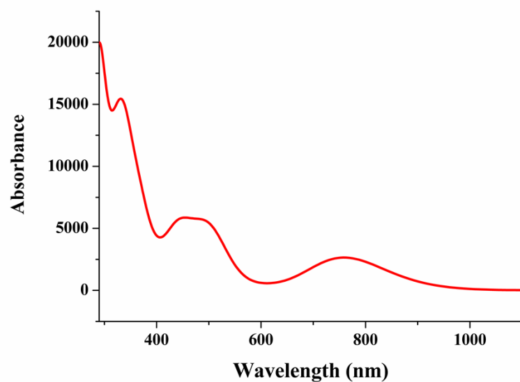
Figure S1. UV-vis-NIR absorption spectra of Sc_2S@C_{72} obtained by BHandHLYP functional
