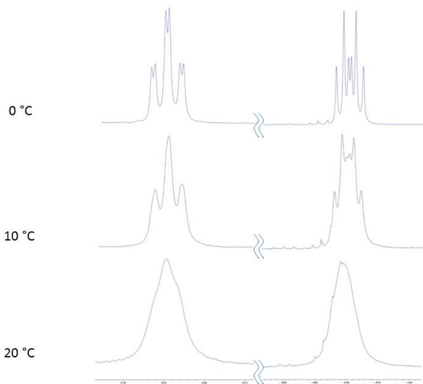
Figure S1. 1 H NMR spectrum of cobalt-methyl resonances of complex 2 (in Tol-d 8 ) at various temperatures.
