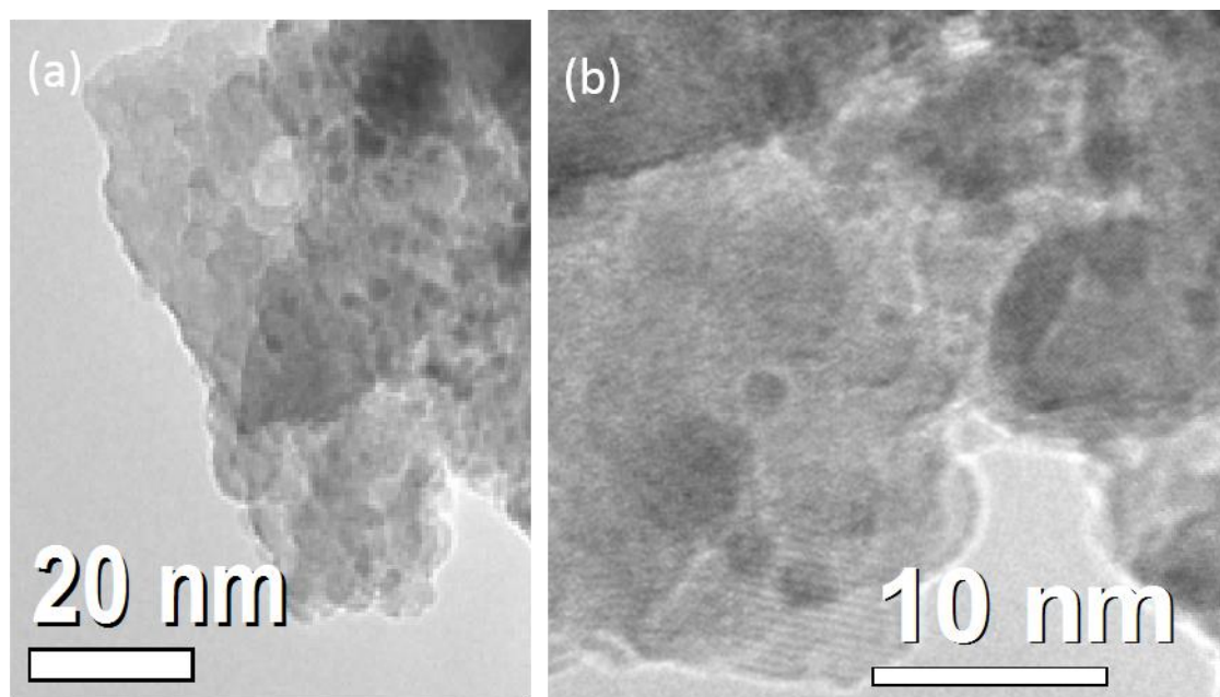
TEM of pattern of LaCoO 3 : Pt (2 wt%)
