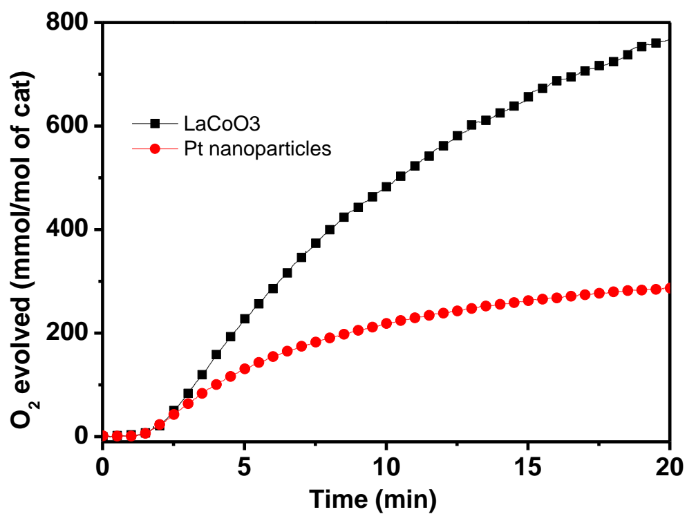
O 2 evolution of the Pt in comparison with LaCoO 3
