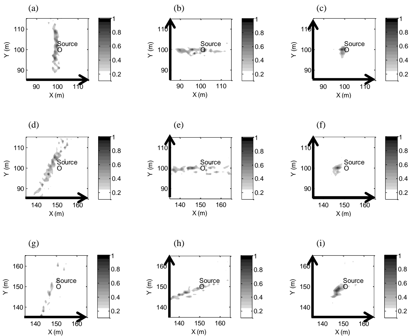
Appendix 1. Reconstruction results at three example source locations after adding 30% of noise to the simulated PIC_{obs} and recalculating the source locations. The grayscale bar represents their relative frequency of occurrence. Rows 1 to 3: Source at (100, 100), (150, 100), and (150, 150), respectively. Columns 1 to 3: Reconstructed by the X-RPM ID , Y-RPM ID , and XY-RPM ID approaches, respectively.
