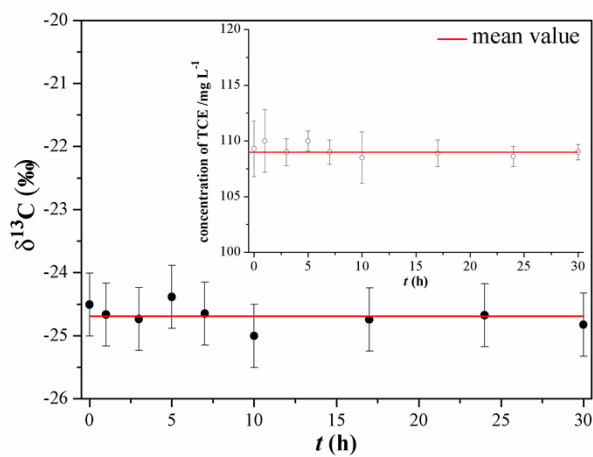
Fig. 1 Trichloroethylene (TCE) carbon isotopic composition ( \delta^{13}\text{C} ) and concentration versus time ( t ) in the Control experiment
