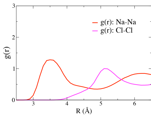
Supplementary Material: Radial distribution of like-charged ion pairs in bulk solution. The red line and magenta lines correspond to the Na-Na and Cl-Cl pairs, respectively.
