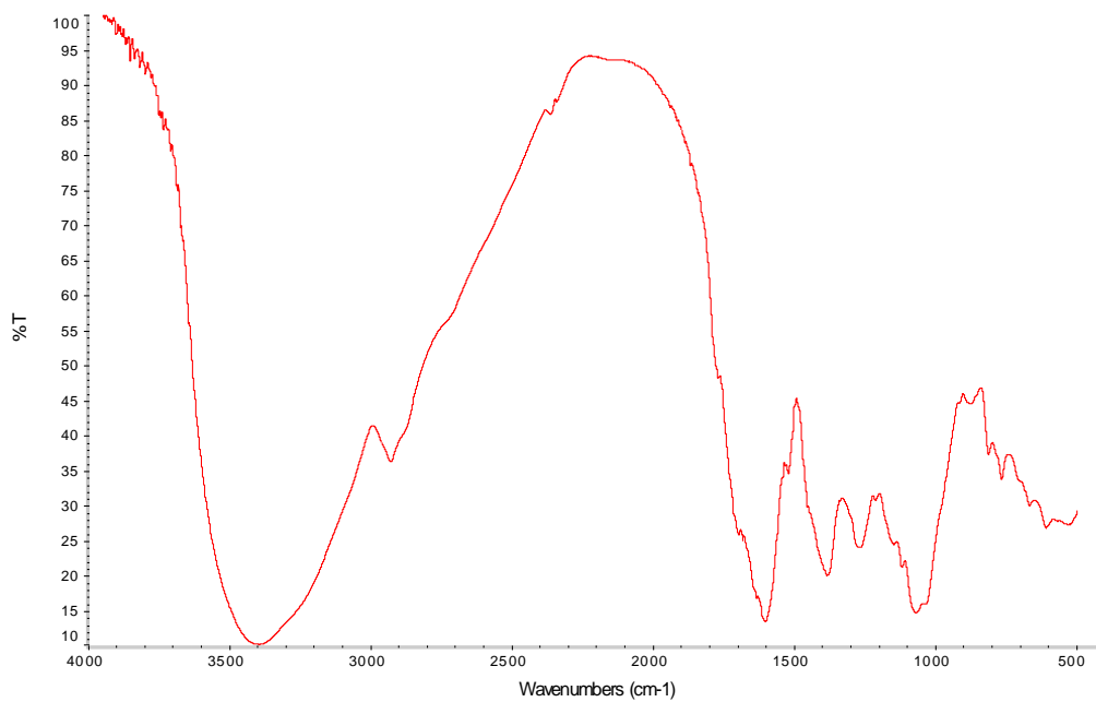
FTIR spectrum of coffee melanoidins in KBr
