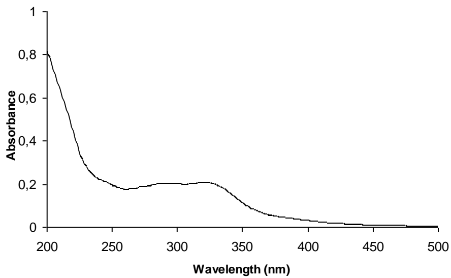
UV-VIS spectrum of coffee melanoidins in distilled water (0.025 mg/ml)
