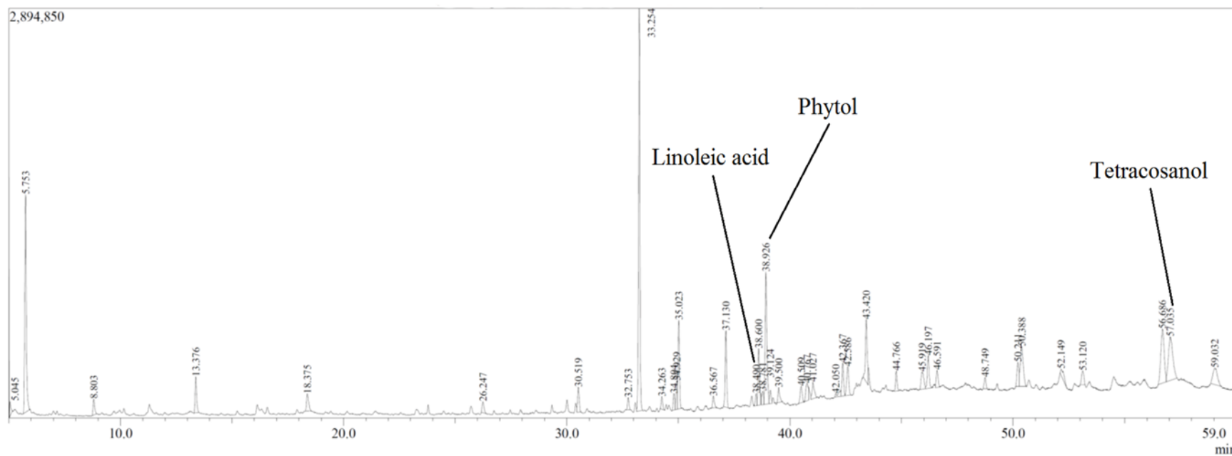
Figure S1. Gas chromatogram of TM-4. The three peaks of linoleic acid, phytol and tetracosanol are indicated, and retention time (min) of three compounds is 38.490, 38.926 and 57.035 min, respectively.
